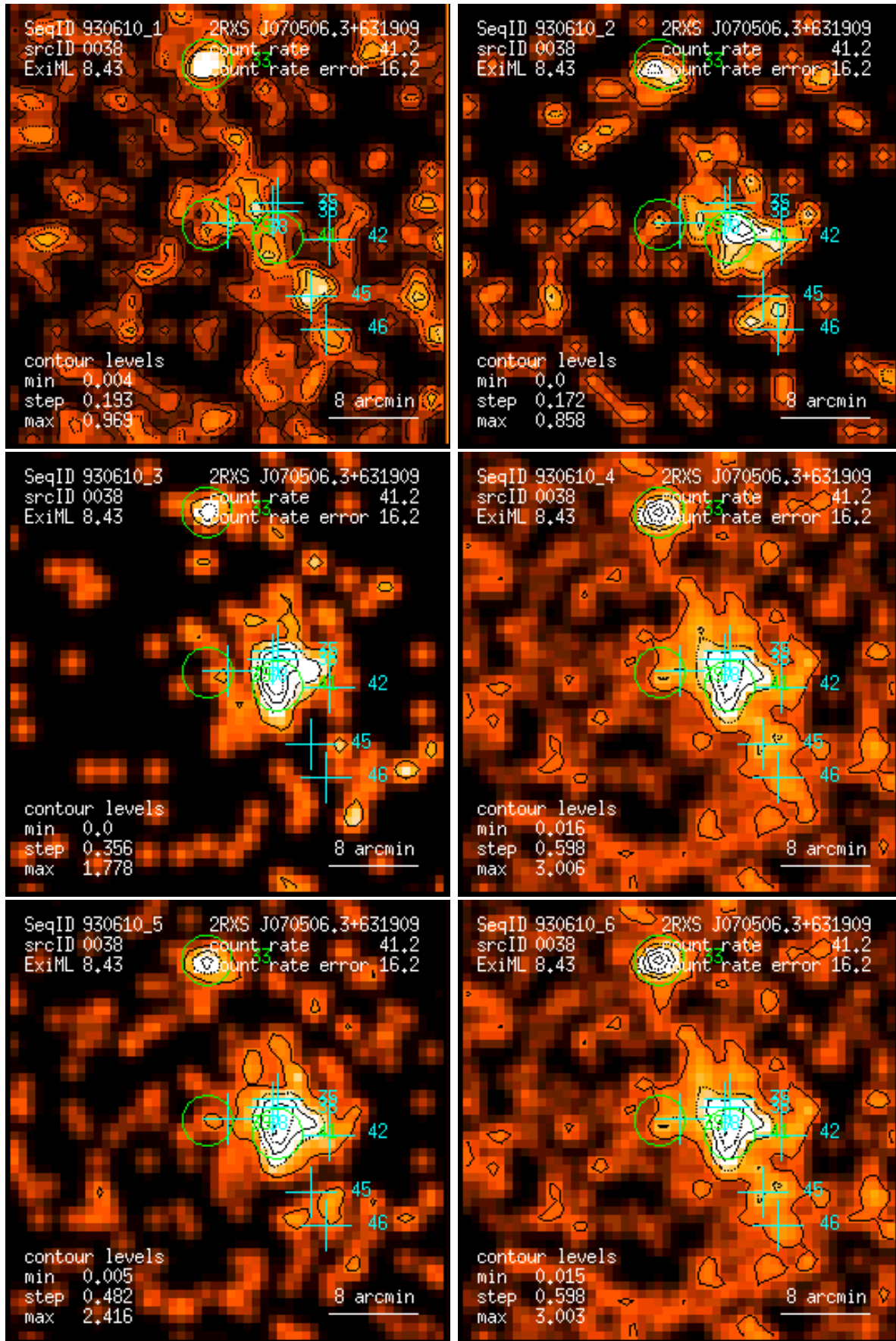
Figure 38: RASS 930610: detection 0038: band rate images, Gaussian filter: (1) PSPC channels 11 – 41, (2) 52 – 90, (3) 91 – 201, (4) 11 – 235, (5) 52 – 201, (6) 11 – 201. Broad band rates in counts/ks. Band rate contour levels in counts/ks/arcmin 2 .
