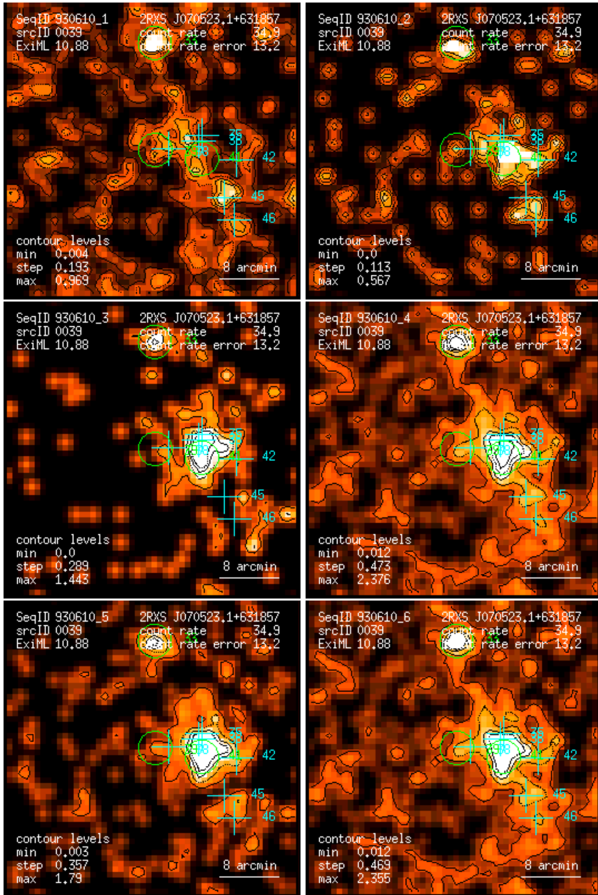
Figure 39: RASS 930610: detection 0039: band rate images, Gaussian filter: (1) PSPC channels 11 – 41, (2) 52 – 90, (3) 91 – 201, (4) 11 – 235, (5) 52 – 201, (6) 11 – 201. Broad band rates in counts/ks. Band rate contour levels in counts/ks/arcmin 2 .
