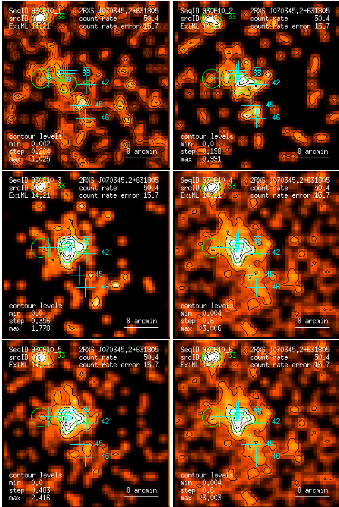
Figure 42: RASS 930610: detection 0042: band rate images, Gaussian filter: (1) PSPC channels 11 – 41, (2) 52 – 90, (3) 91 – 201, (4) 11 – 235, (5) 52 – 201, (6) 11 – 201. Broad band rates in counts/ks. Band rate contour levels in counts/ks/arcmin 2 .
