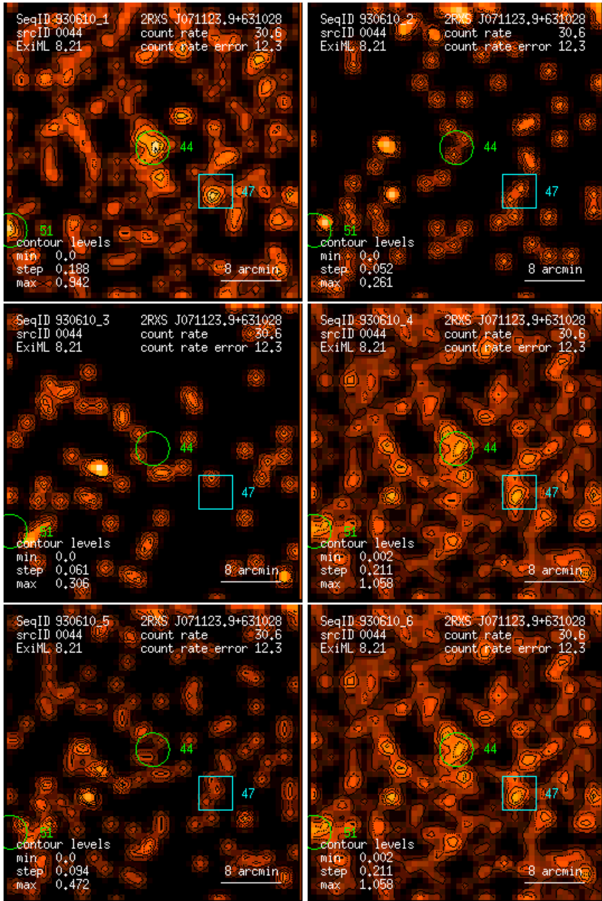
Figure 44: RASS 930610: detection 0044: band rate images, Gaussian filter: (1) PSPC channels 11 – 41, (2) 52 – 90, (3) 91 – 201, (4) 11 – 235, (5) 52 – 201, (6) 11 – 201. Broad band rates in counts/ks. Band rate contour levels in counts/ks/arcmin 2 .
