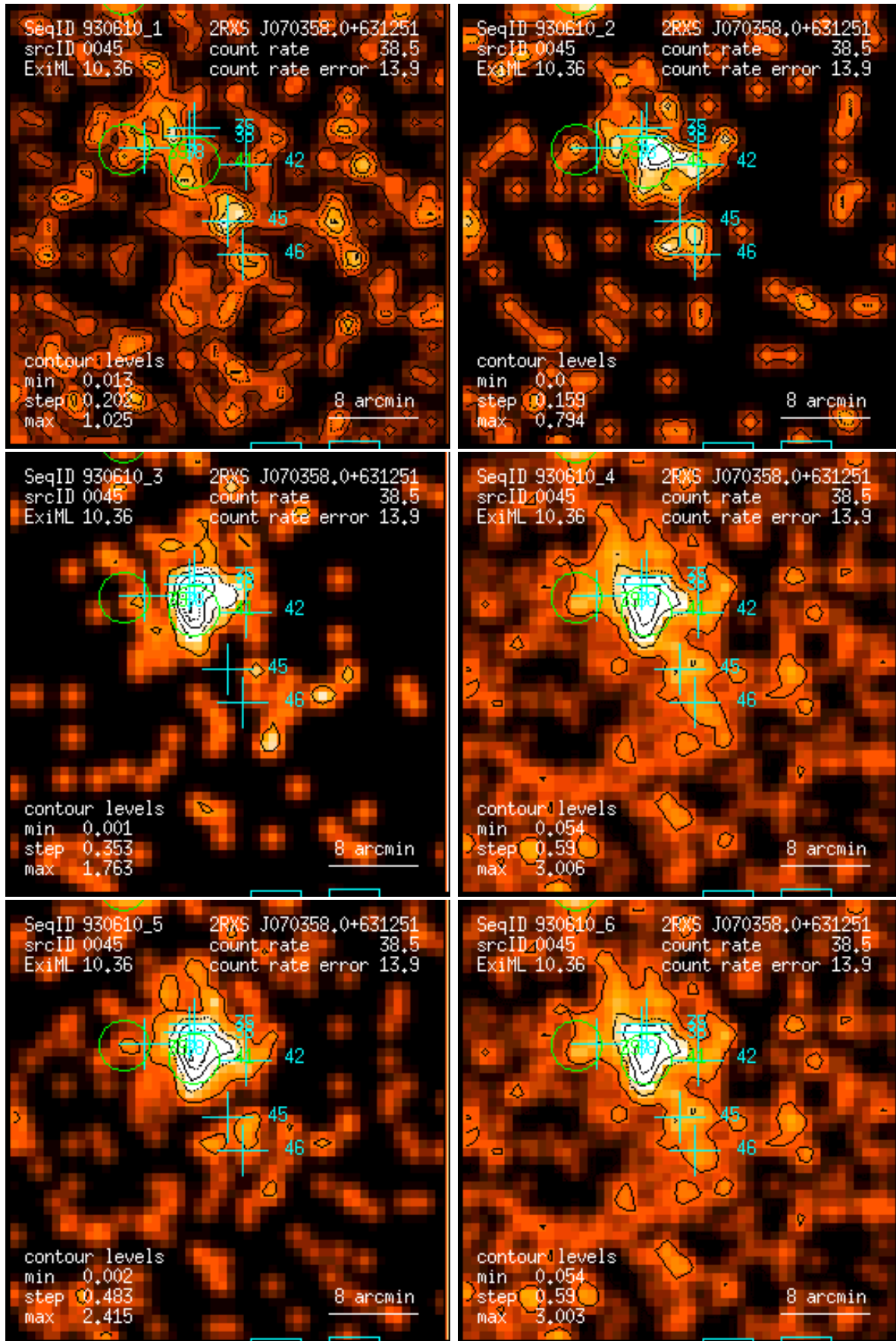
Figure 45: RASS 930610: detection 0045: band rate images, Gaussian filter: (1) PSPC channels 11 – 41, (2) 52 – 90, (3) 91 – 201, (4) 11 – 235, (5) 52 – 201, (6) 11 – 201. Broad band rates in counts/ks. Band rate contour levels in counts/ks/arcmin 2 .
