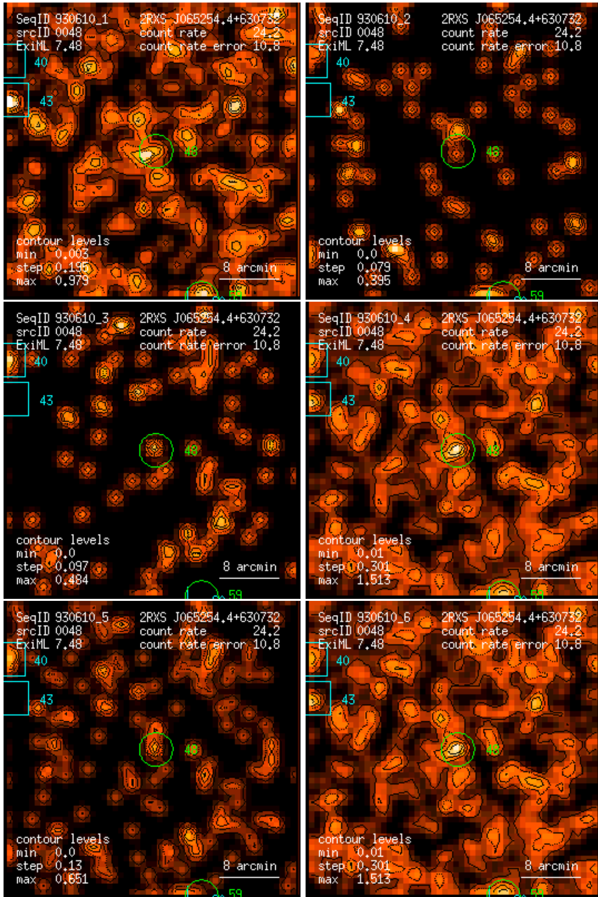
Figure 48: RASS 930610: detection 0048: band rate images, Gaussian filter: (1) PSPC channels 11 – 41, (2) 52 – 90, (3) 91 – 201, (4) 11 – 235, (5) 52 – 201, (6) 11 – 201. Broad band rates in counts/ks. Band rate contour levels in counts/ks/arcmin 2 .
