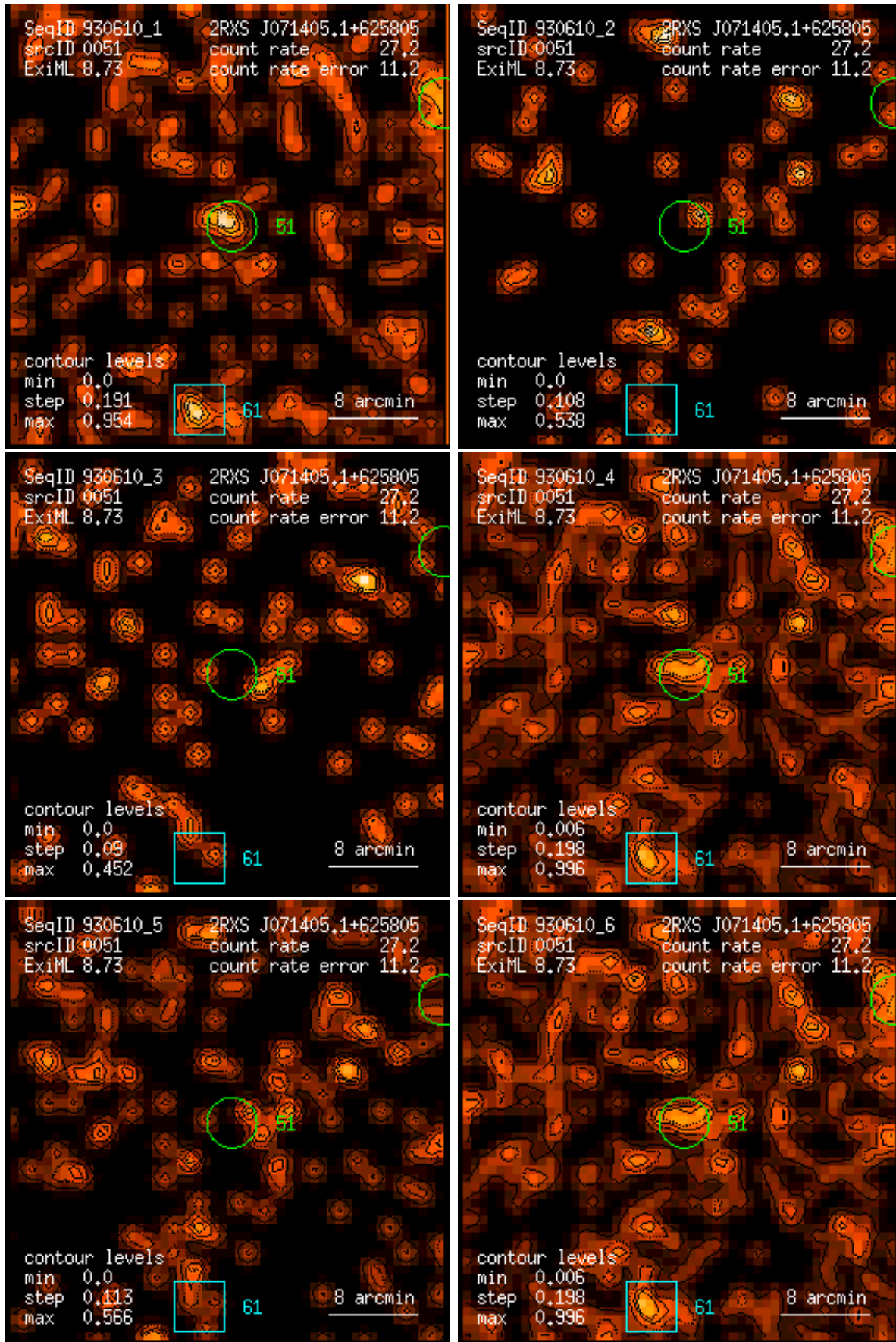
Figure 51: RASS 930610: detection 0051: band rate images, Gaussian filter: (1) PSPC channels 11 – 41, (2) 52 – 90, (3) 91 – 201, (4) 11 – 235, (5) 52 – 201, (6) 11 – 201. Broad band rates in counts/ks. Band rate contour levels in counts/ks/arcmin 2 .
