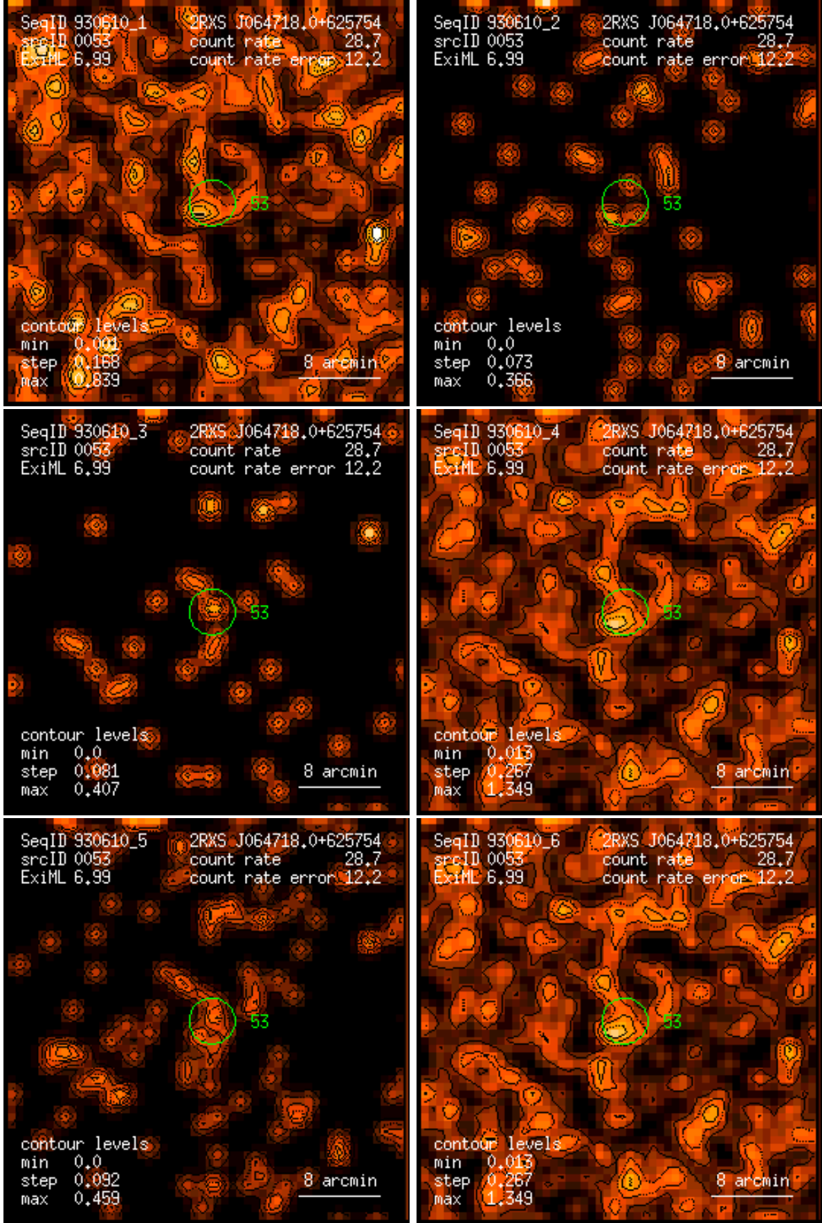
Figure 53: RASS 930610: detection 0053: band rate images, Gaussian filter: (1) PSPC channels 11 – 41, (2) 52 – 90, (3) 91 – 201, (4) 11 – 235, (5) 52 – 201, (6) 11 – 201. Broad band rates in counts/ks. Band rate contour levels in counts/ks/arcmin 2 .
