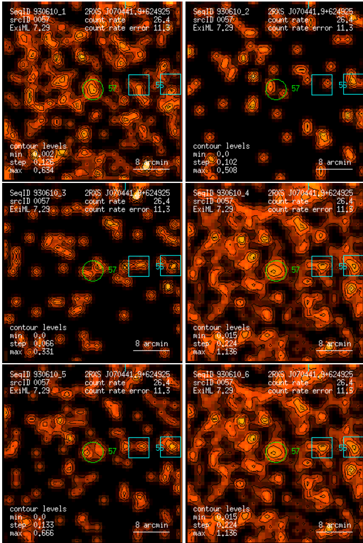
Figure 57: RASS 930610: detection 0057: band rate images, Gaussian filter: (1) PSPC channels 11 – 41, (2) 52 – 90, (3) 91 – 201, (4) 11 – 235, (5) 52 – 201, (6) 11 – 201. Broad band rates in counts/ks. Band rate contour levels in counts/ks/arcmin 2 .
