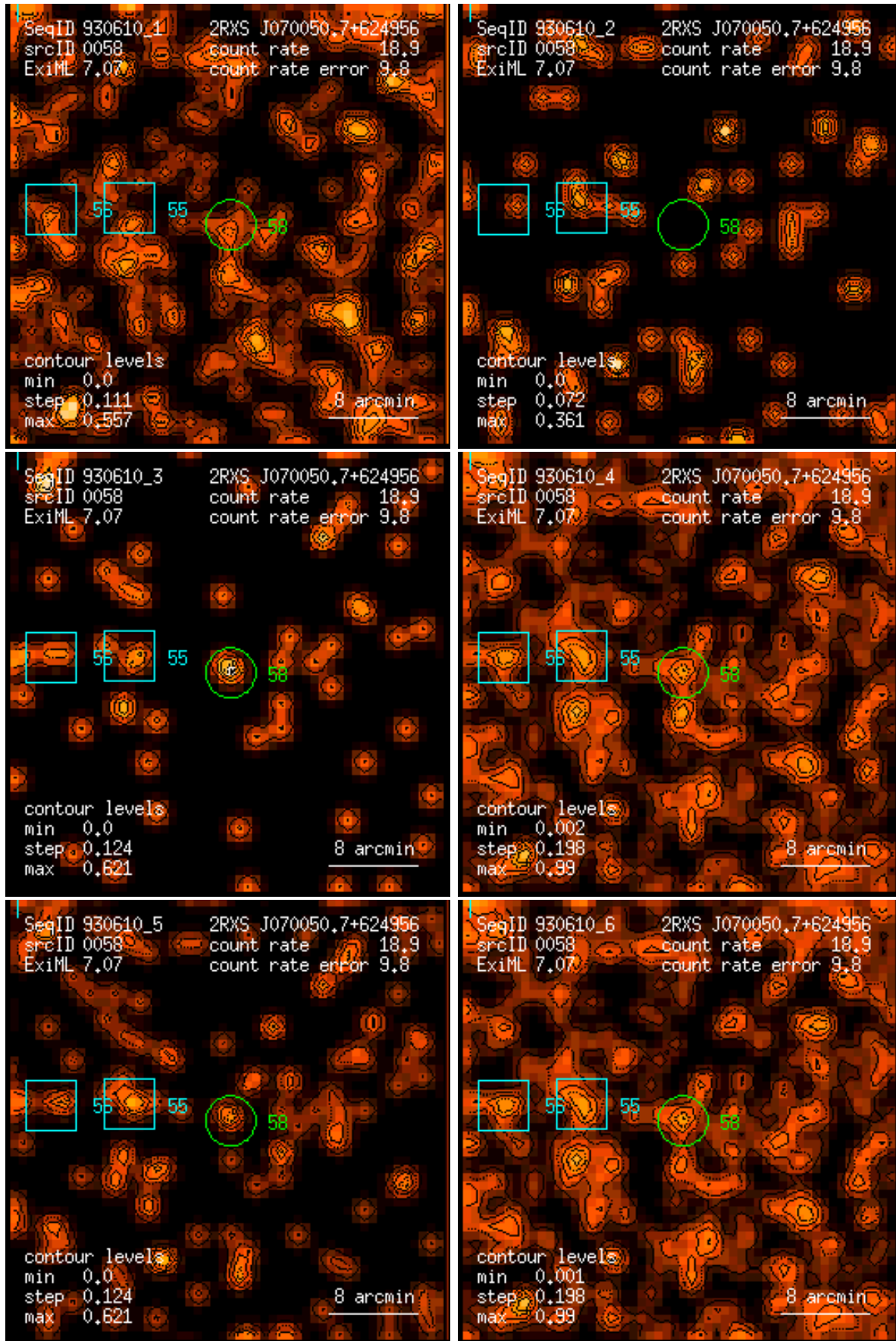
Figure 58: RASS 930610: detection 0058: band rate images, Gaussian filter: (1) PSPC channels 11 – 41, (2) 52 – 90, (3) 91 – 201, (4) 11 – 235, (5) 52 – 201, (6) 11 – 201. Broad band rates in counts/ks. Band rate contour levels in counts/ks/arcmin 2 .
