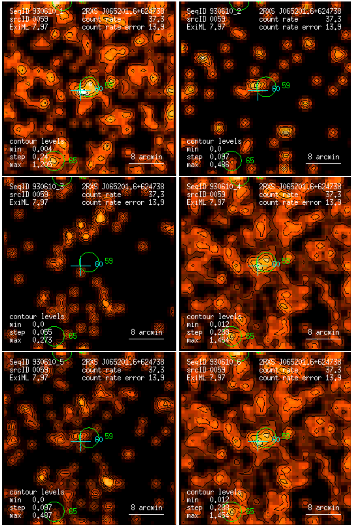
Figure 59: RASS 930610: detection 0059: band rate images, Gaussian filter: (1) PSPC channels 11 – 41, (2) 52 – 90, (3) 91 – 201, (4) 11 – 235, (5) 52 – 201, (6) 11 – 201. Broad band rates in counts/ks. Band rate contour levels in counts/ks/arcmin 2 .
