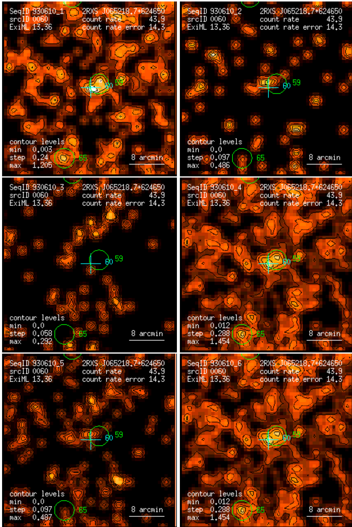
Figure 60: RASS 930610: detection 0060: band rate images, Gaussian filter: (1) PSPC channels 11 – 41, (2) 52 – 90, (3) 91 – 201, (4) 11 – 235, (5) 52 – 201, (6) 11 – 201. Broad band rates in counts/ks. Band rate contour levels in counts/ks/arcmin 2 .
