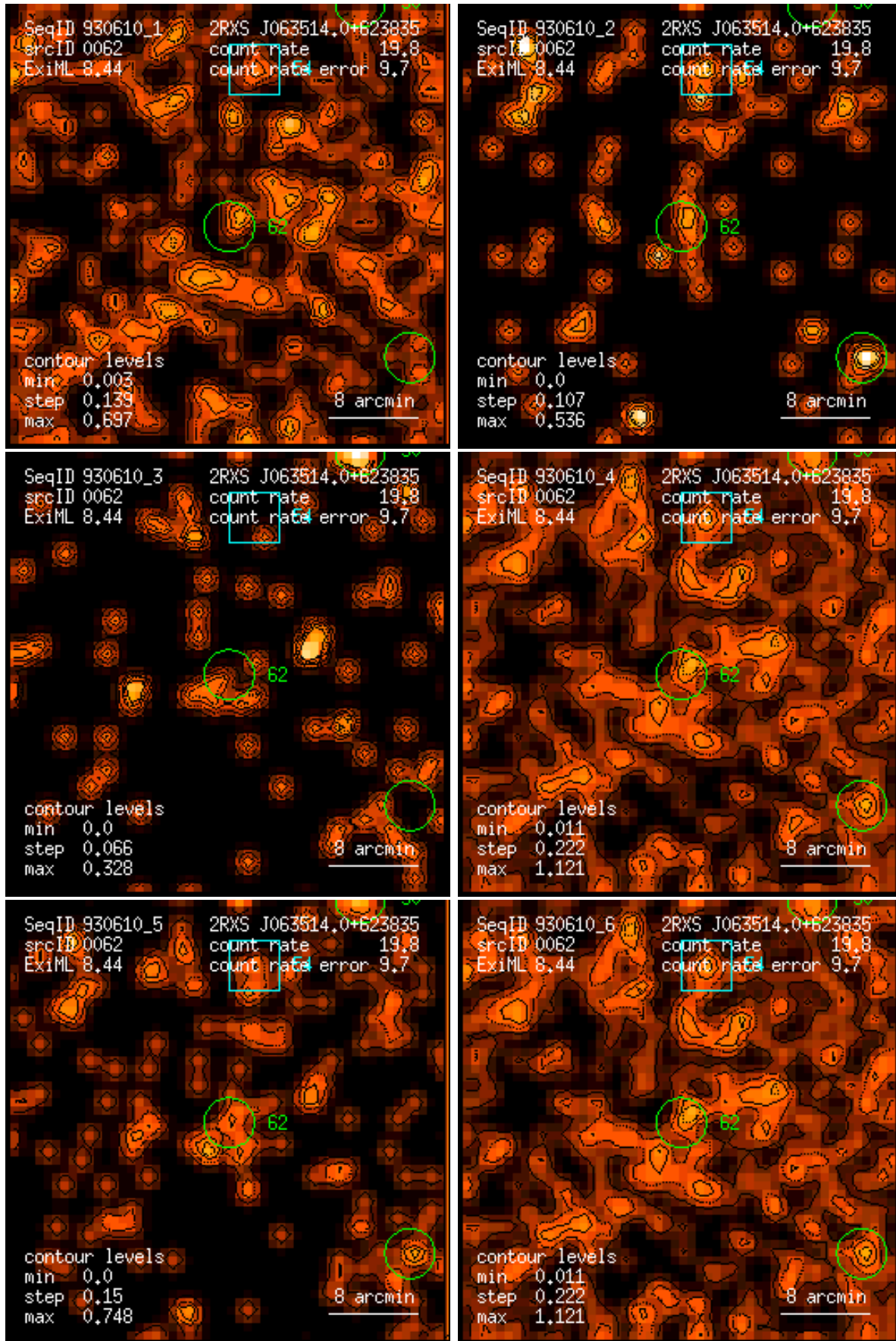
Figure 62: RASS 930610: detection 0062: band rate images, Gaussian filter: (1) PSPC channels 11 – 41, (2) 52 – 90, (3) 91 – 201, (4) 11 – 235, (5) 52 – 201, (6) 11 – 201. Broad band rates in counts/ks. Band rate contour levels in counts/ks/arcmin 2 .
