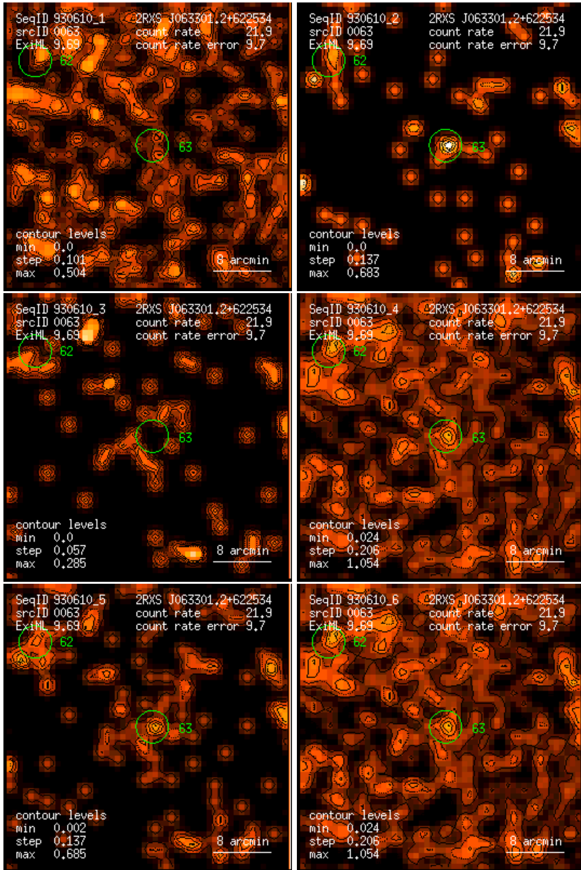
Figure 63: RASS 930610: detection 0063: band rate images, Gaussian filter: (1) PSPC channels 11 – 41, (2) 52 – 90, (3) 91 – 201, (4) 11 – 235, (5) 52 – 201, (6) 11 – 201. Broad band rates in counts/ks. Band rate contour levels in counts/ks/arcmin 2 .
