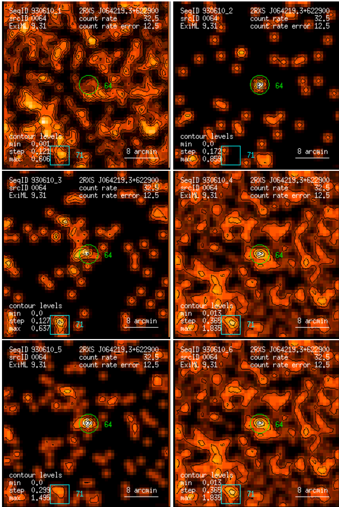
Figure 64: RASS 930610: detection 0064: band rate images, Gaussian filter: (1) PSPC channels 11 – 41, (2) 52 – 90, (3) 91 – 201, (4) 11 – 235, (5) 52 – 201, (6) 11 – 201. Broad band rates in counts/ks. Band rate contour levels in counts/ks/arcmin 2 .
