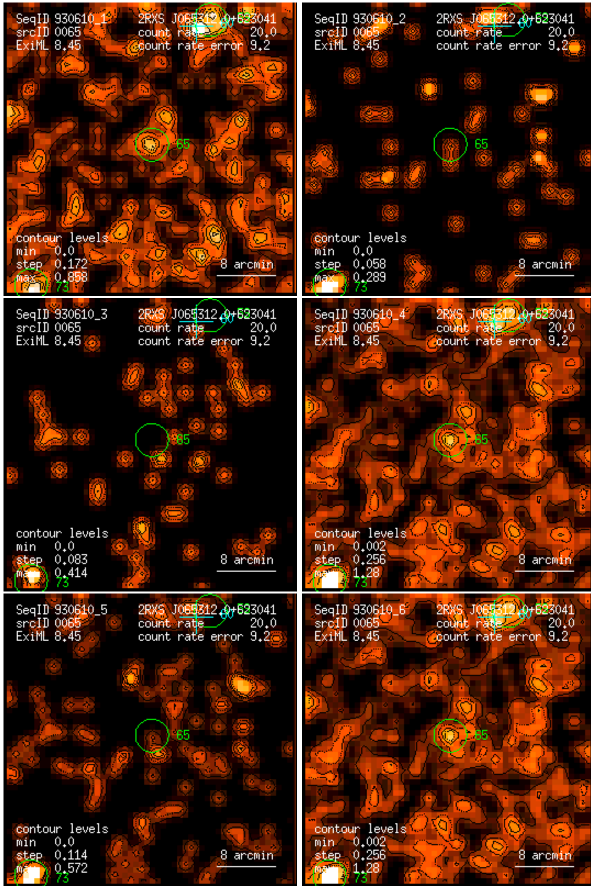
Figure 65: RASS 930610: detection 0065: band rate images, Gaussian filter: (1) PSPC channels 11 – 41, (2) 52 – 90, (3) 91 – 201, (4) 11 – 235, (5) 52 – 201, (6) 11 – 201. Broad band rates in counts/ks. Band rate contour levels in counts/ks/arcmin 2 .
