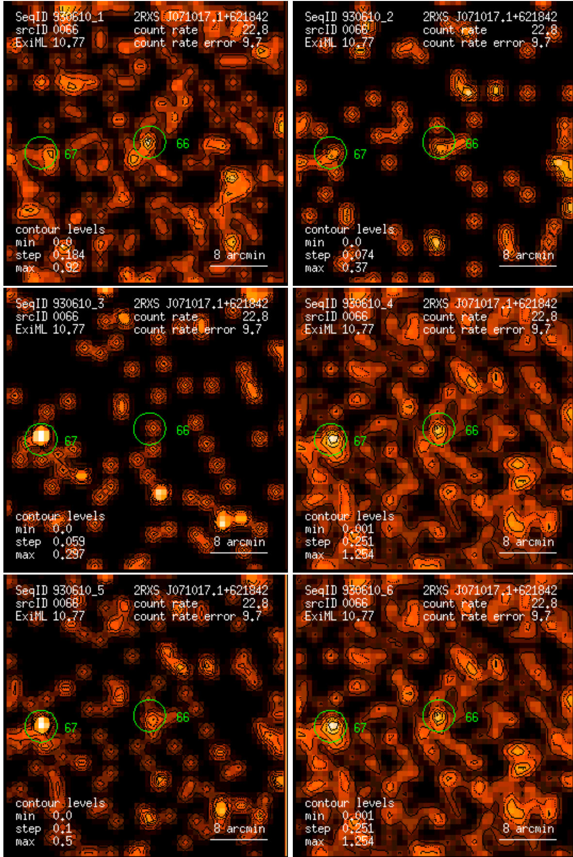
Figure 66: RASS 930610: detection 0066: band rate images, Gaussian filter: (1) PSPC channels 11 – 41, (2) 52 – 90, (3) 91 – 201, (4) 11 – 235, (5) 52 – 201, (6) 11 – 201. Broad band rates in counts/ks. Band rate contour levels in counts/ks/arcmin 2 .
