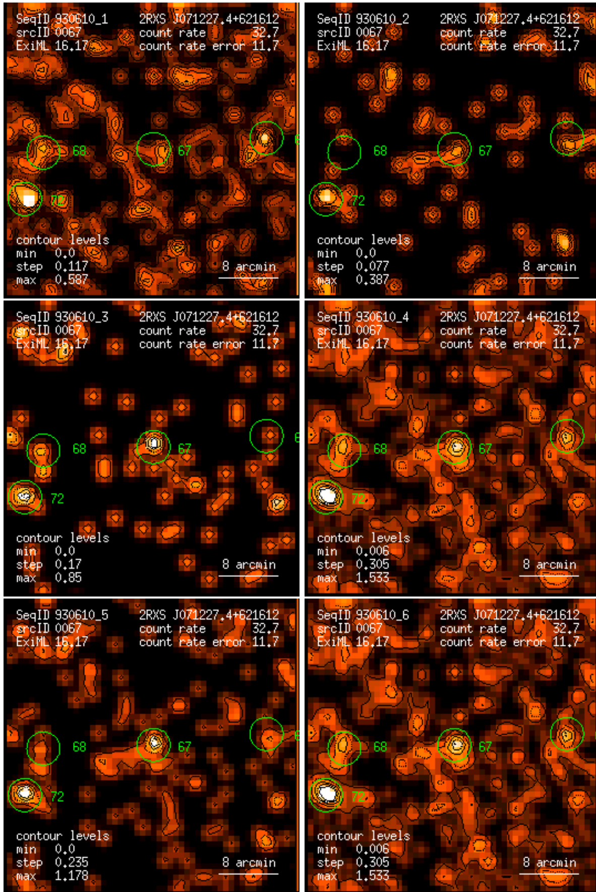
Figure 67: RASS 930610: detection 0067: band rate images, Gaussian filter: (1) PSPC channels 11 – 41, (2) 52 – 90, (3) 91 – 201, (4) 11 – 235, (5) 52 – 201, (6) 11 – 201. Broad band rates in counts/ks. Band rate contour levels in counts/ks/arcmin 2 .
