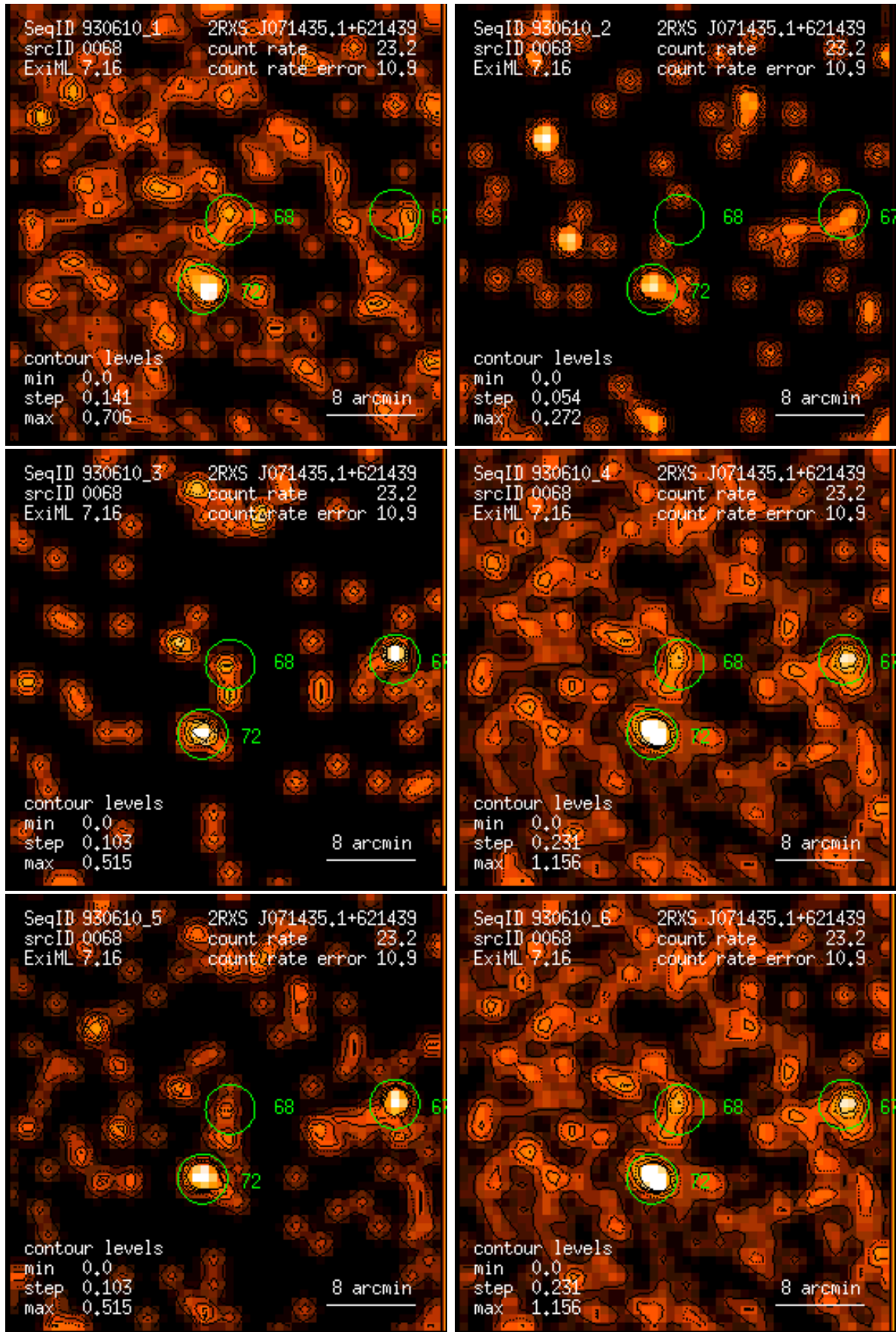
Figure 68: RASS 930610: detection 0068: band rate images, Gaussian filter: (1) PSPC channels 11 – 41, (2) 52 – 90, (3) 91 – 201, (4) 11 – 235, (5) 52 – 201, (6) 11 – 201. Broad band rates in counts/ks. Band rate contour levels in counts/ks/arcmin 2 .
