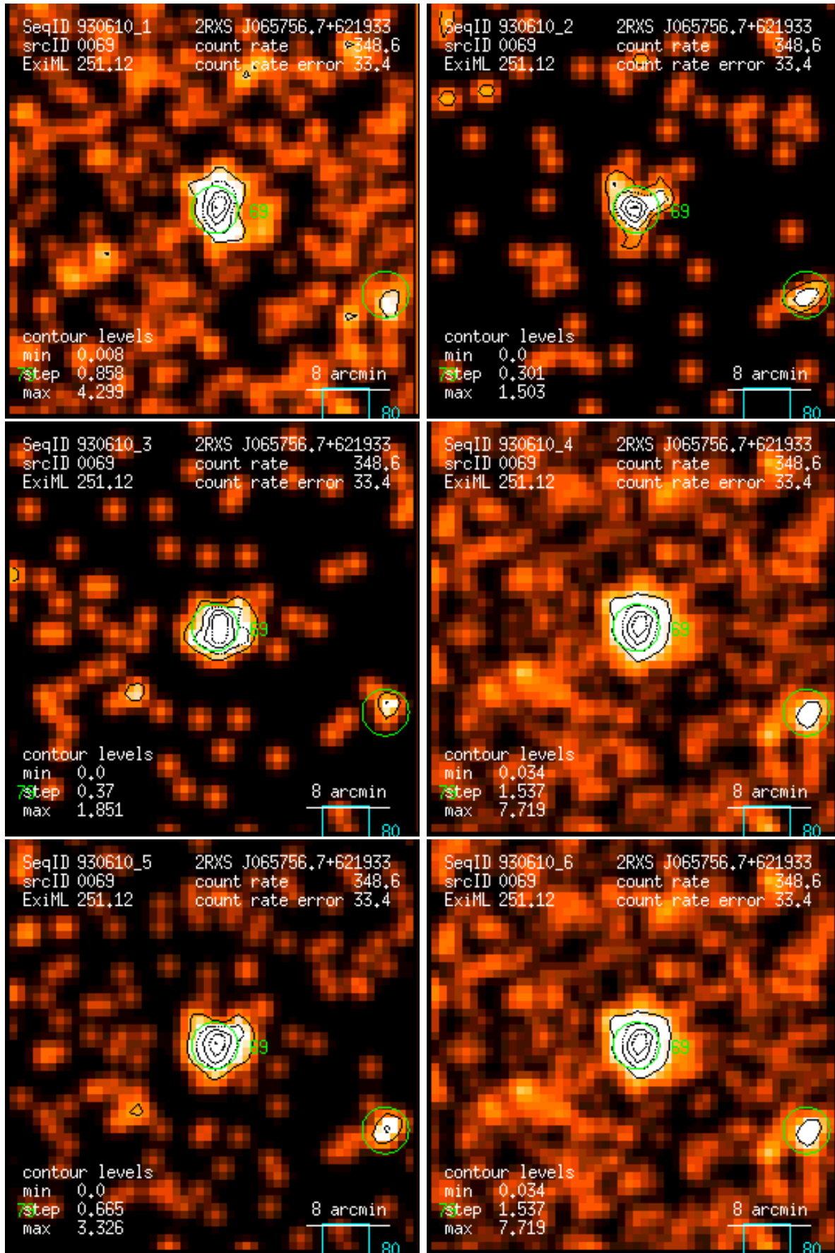
Figure 69: RASS 930610: detection 0069: band rate images, Gaussian filter: (1) PSPC channels 11 – 41, (2) 52 – 90, (3) 91 – 201, (4) 11 – 235, (5) 52 – 201, (6) 11 – 201. Broad band rates in counts/ks. Band rate contour levels in counts/ks/arcmin 2 .
