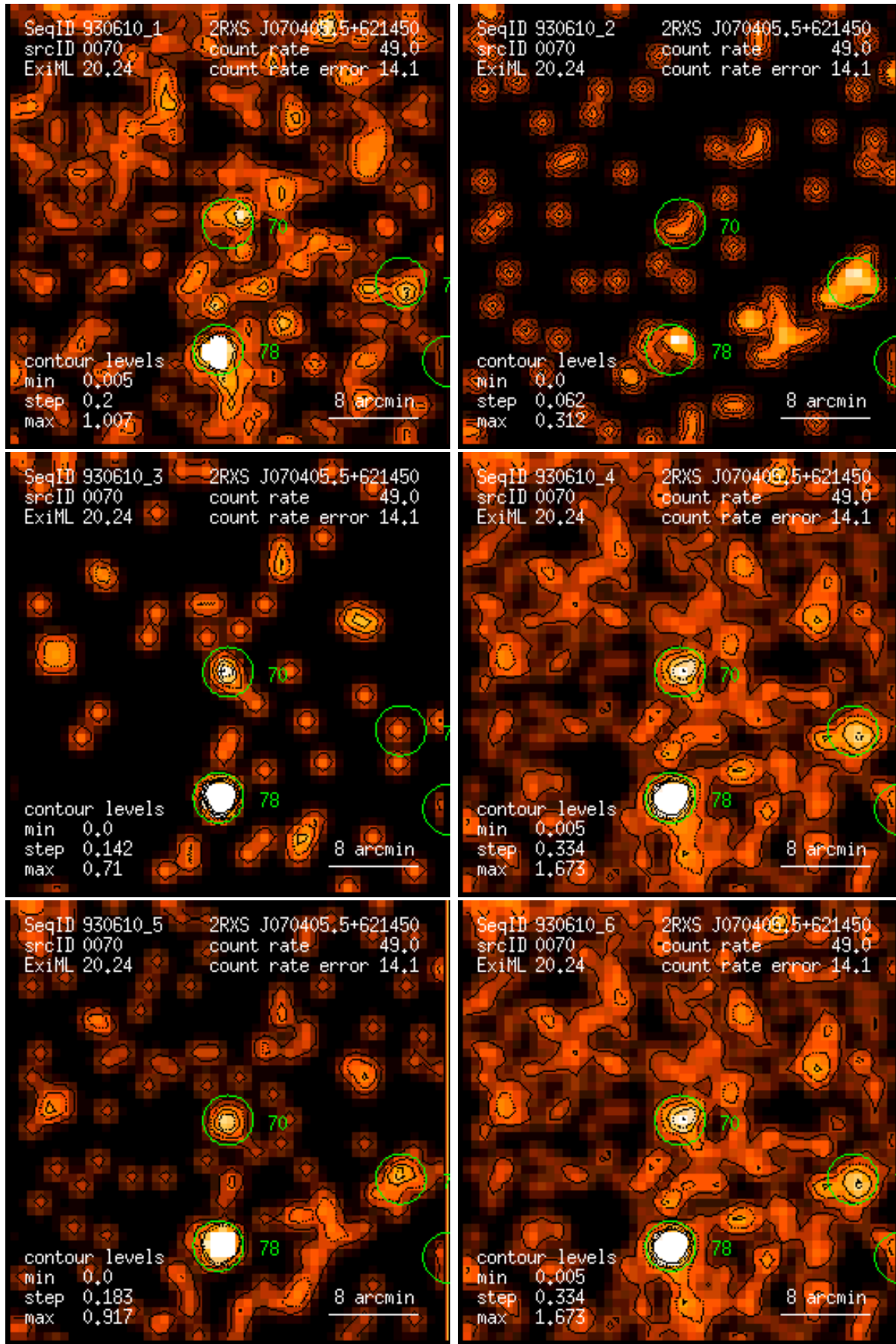
Figure 70: RASS 930610: detection 0070: band rate images, Gaussian filter: (1) PSPC channels 11 – 41, (2) 52 – 90, (3) 91 – 201, (4) 11 – 235, (5) 52 – 201, (6) 11 – 201. Broad band rates in counts/ks. Band rate contour levels in counts/ks/arcmin 2 .
