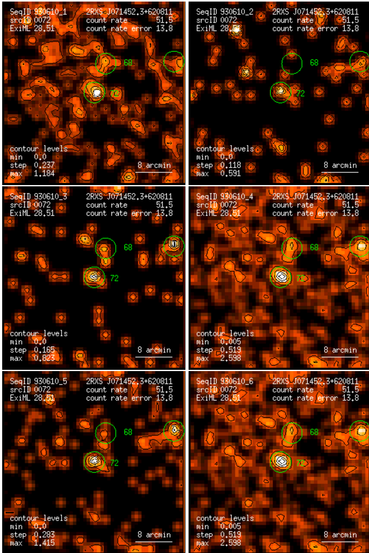
Figure 72: RASS 930610: detection 0072: band rate images, Gaussian filter: (1) PSPC channels 11 – 41, (2) 52 – 90, (3) 91 – 201, (4) 11 – 235, (5) 52 – 201, (6) 11 – 201. Broad band rates in counts/ks. Band rate contour levels in counts/ks/arcmin 2 .
