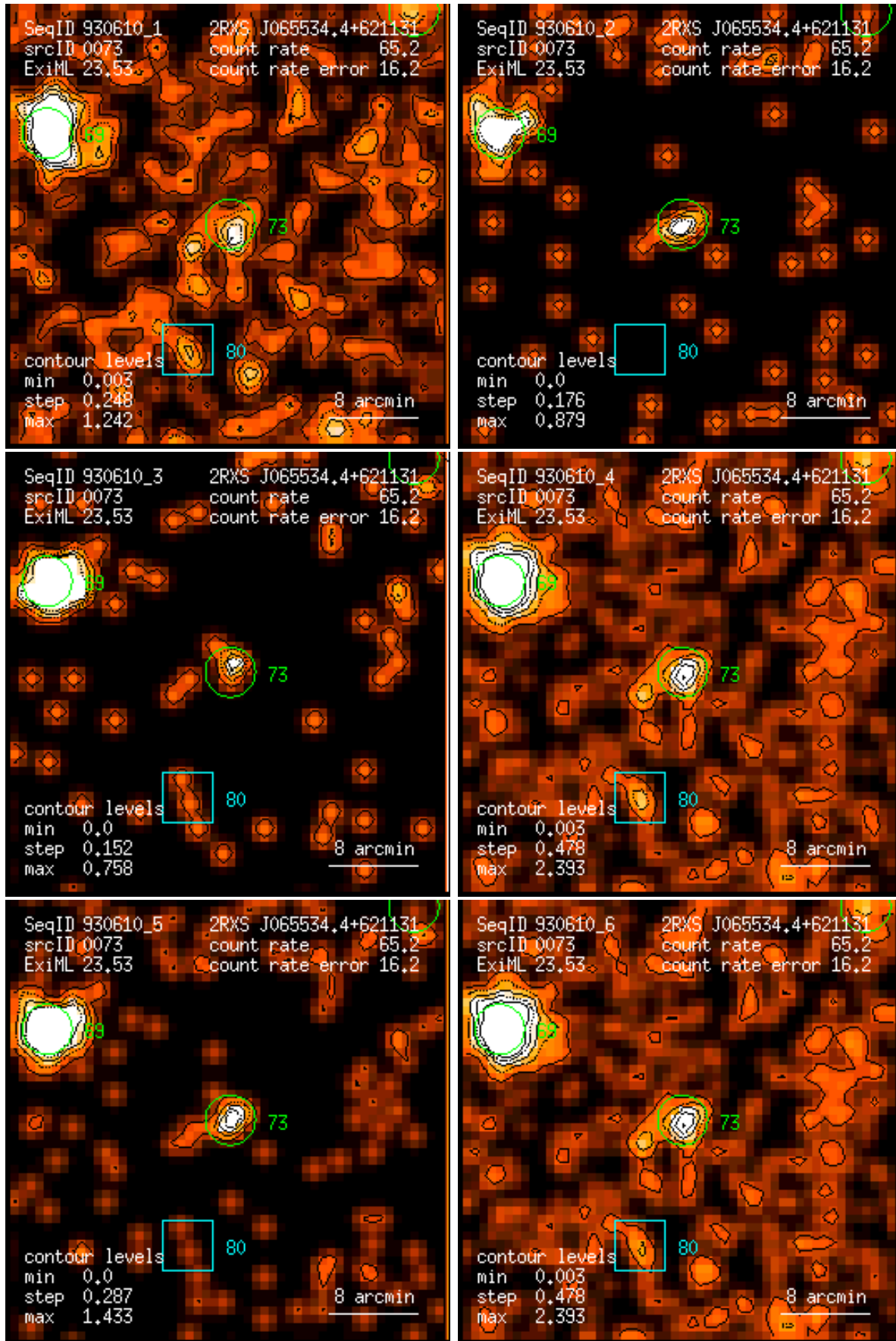
Figure 73: RASS 930610: detection 0073: band rate images, Gaussian filter: (1) PSPC channels 11 – 41, (2) 52 – 90, (3) 91 – 201, (4) 11 – 235, (5) 52 – 201, (6) 11 – 201. Broad band rates in counts/ks. Band rate contour levels in counts/ks/arcmin 2 .
