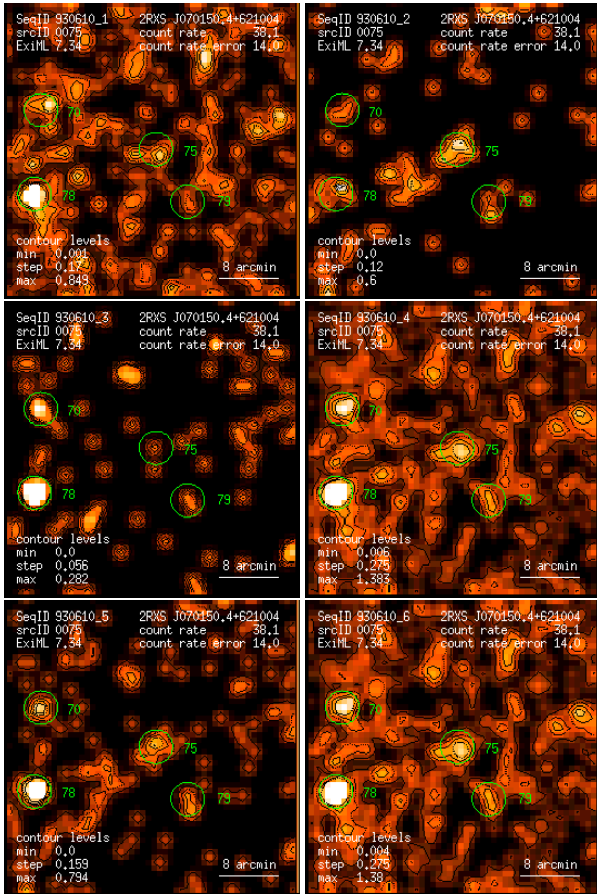
Figure 75: RASS 930610: detection 0075: band rate images, Gaussian filter: (1) PSPC channels 11 – 41, (2) 52 – 90, (3) 91 – 201, (4) 11 – 235, (5) 52 – 201, (6) 11 – 201. Broad band rates in counts/ks. Band rate contour levels in counts/ks/arcmin 2 .
