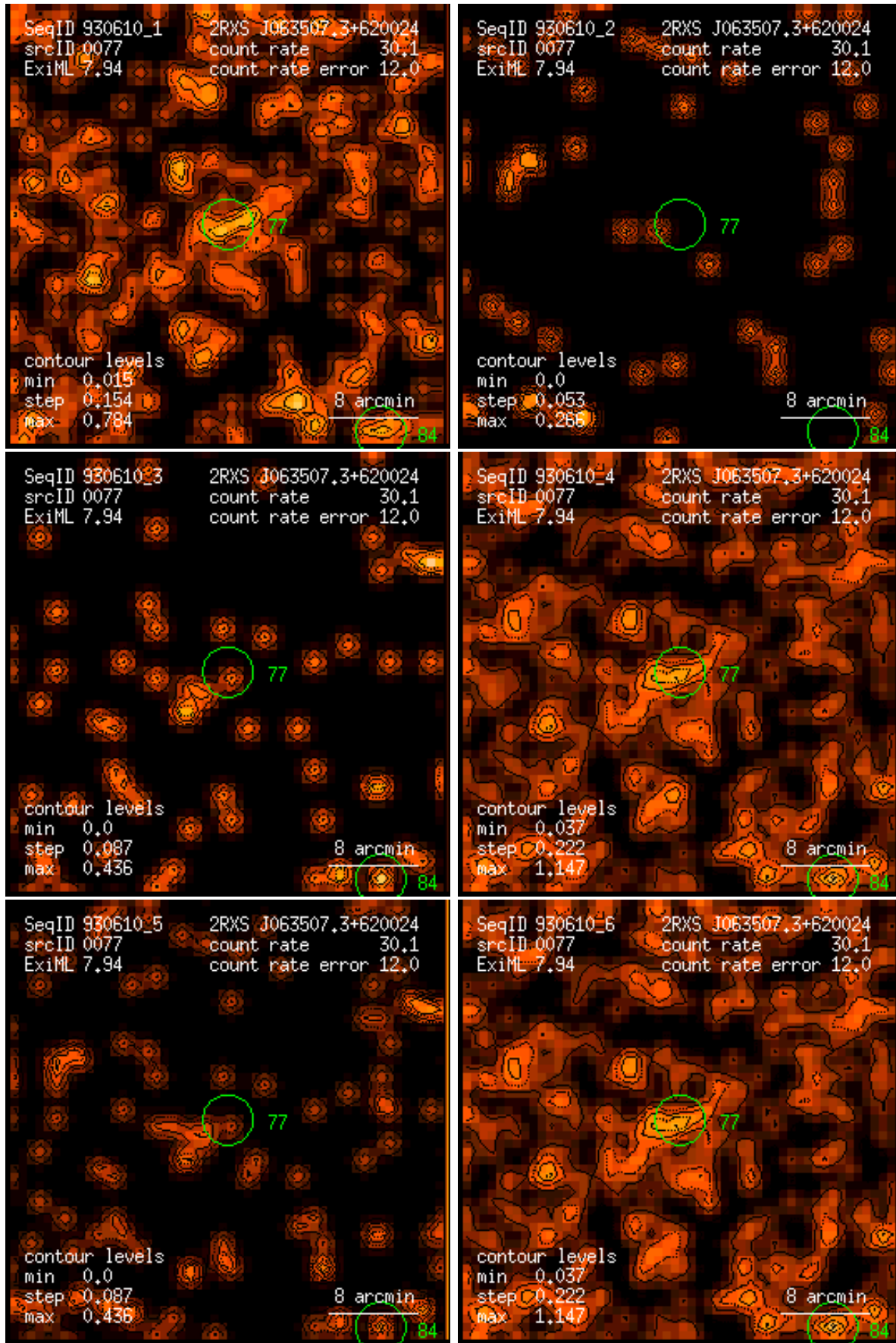
Figure 77: RASS 930610: detection 0077: band rate images, Gaussian filter: (1) PSPC channels 11 – 41, (2) 52 – 90, (3) 91 – 201, (4) 11 – 235, (5) 52 – 201, (6) 11 – 201. Broad band rates in counts/ks. Band rate contour levels in counts/ks/arcmin 2 .
