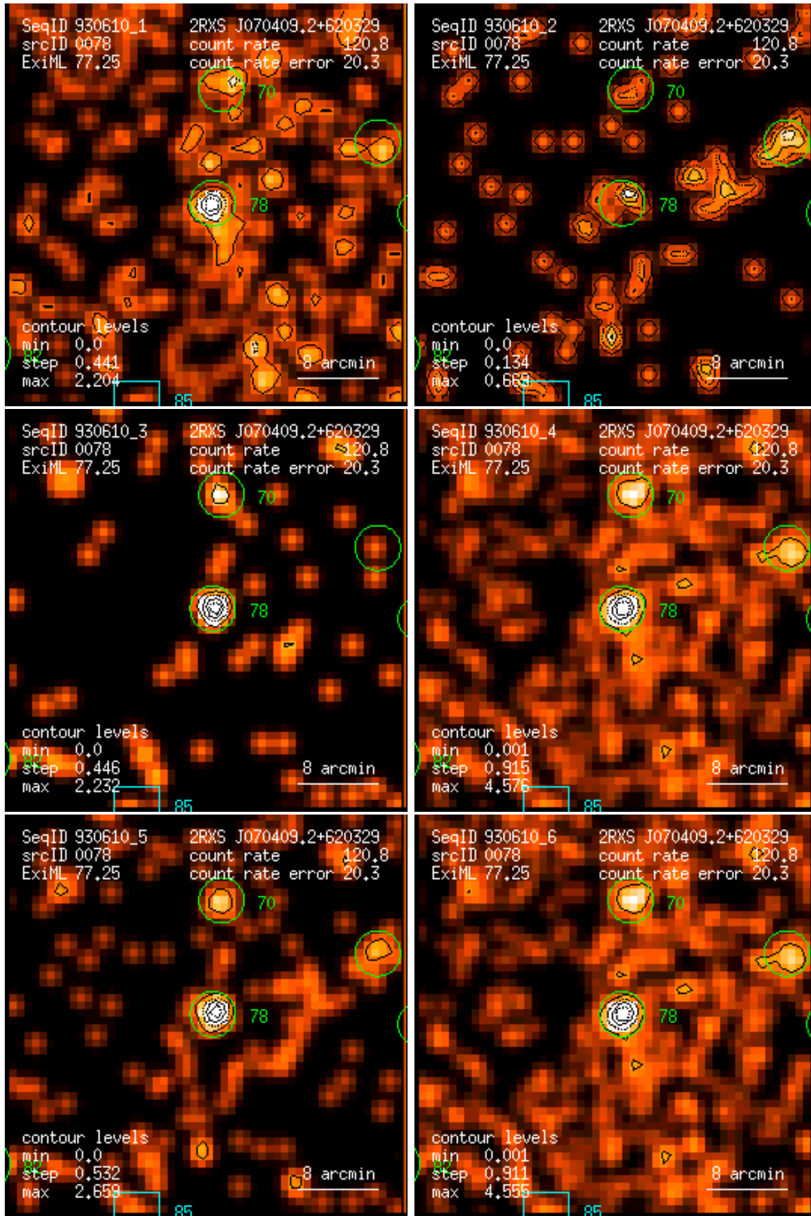
Figure 78: RASS 930610: detection 0078: band rate images, Gaussian filter: (1) PSPC channels 11 – 41, (2) 52 – 90, (3) 91 – 201, (4) 11 – 235, (5) 52 – 201, (6) 11 – 201. Broad band rates in counts/ks. Band rate contour levels in counts/ks/arcmin 2 .
