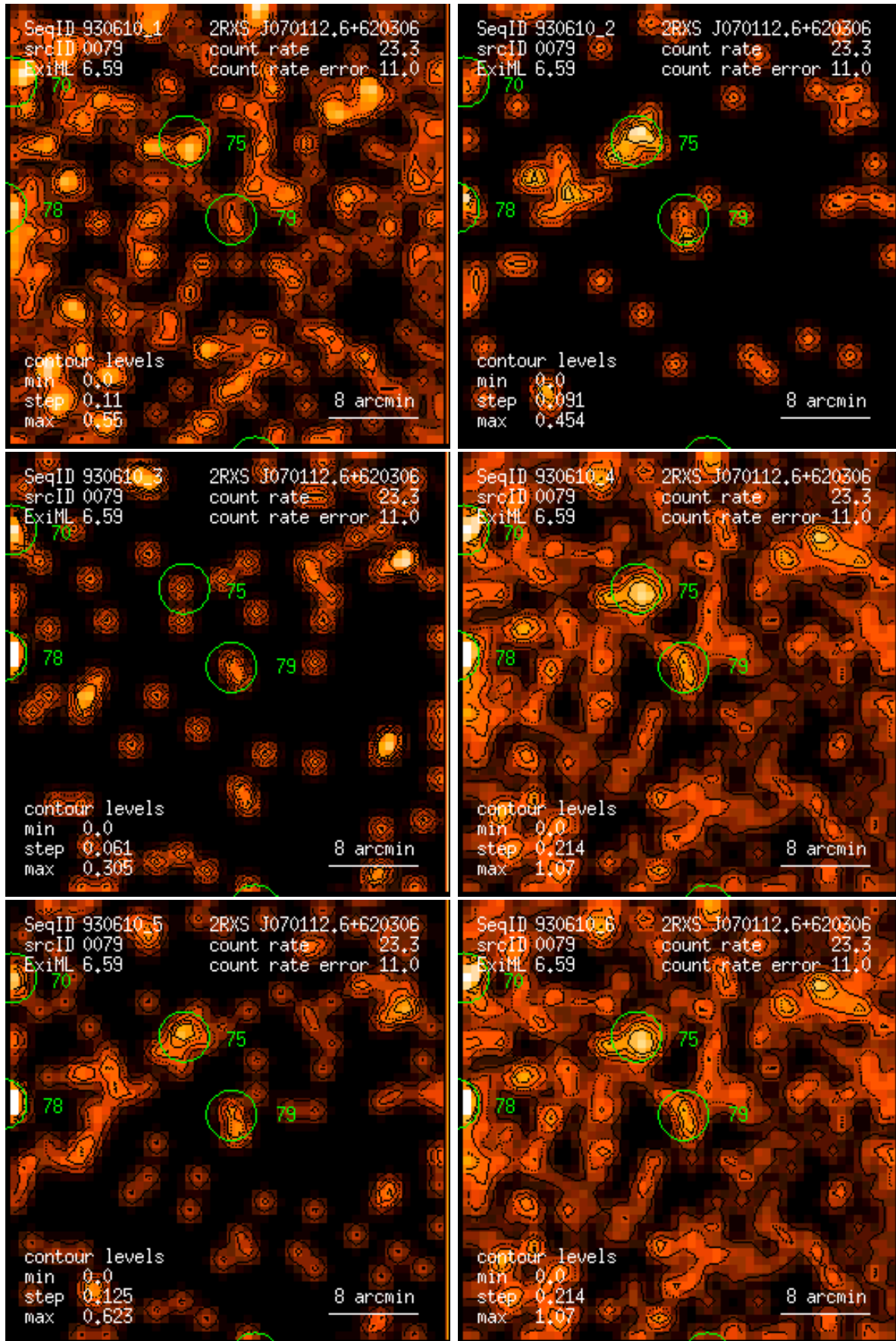
Figure 79: RASS 930610: detection 0079: band rate images, Gaussian filter: (1) PSPC channels 11 – 41, (2) 52 – 90, (3) 91 – 201, (4) 11 – 235, (5) 52 – 201, (6) 11 – 201. Broad band rates in counts/ks. Band rate contour levels in counts/ks/arcmin 2 .
