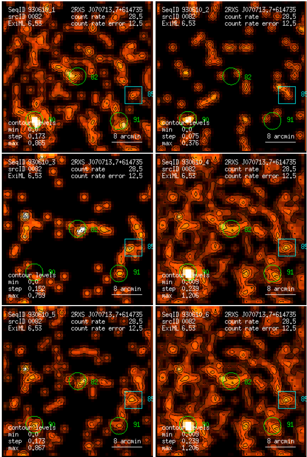
Figure 82: RASS 930610: detection 0082: band rate images, Gaussian filter: (1) PSPC channels 11 – 41, (2) 52 – 90, (3) 91 – 201, (4) 11 – 235, (5) 52 – 201, (6) 11 – 201. Broad band rates in counts/ks. Band rate contour levels in counts/ks/arcmin 2 .
