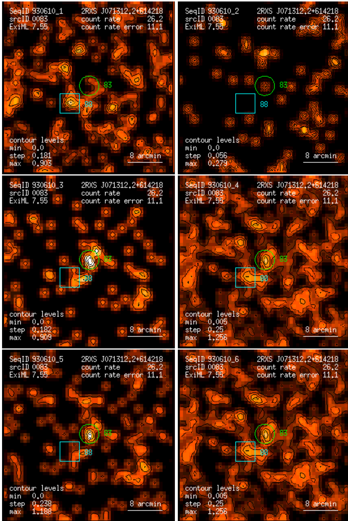
Figure 83: RASS 930610: detection 0083: band rate images, Gaussian filter: (1) PSPC channels 11 – 41, (2) 52 – 90, (3) 91 – 201, (4) 11 – 235, (5) 52 – 201, (6) 11 – 201. Broad band rates in counts/ks. Band rate contour levels in counts/ks/arcmin 2 .
