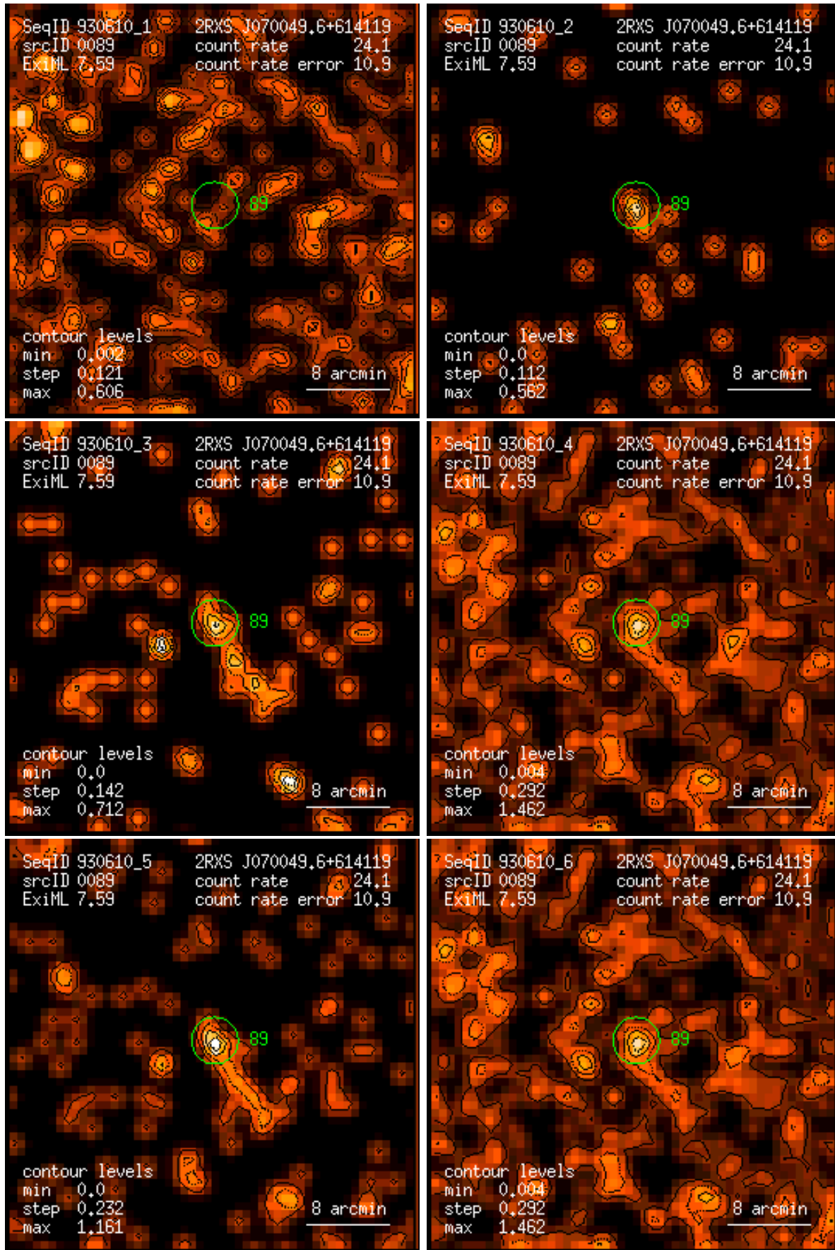
Figure 89: RASS 930610: detection 0089: band rate images, Gaussian filter: (1) PSPC channels 11 – 41, (2) 52 – 90, (3) 91 – 201, (4) 11 – 235, (5) 52 – 201, (6) 11 – 201. Broad band rates in counts/ks. Band rate contour levels in counts/ks/arcmin 2 .
