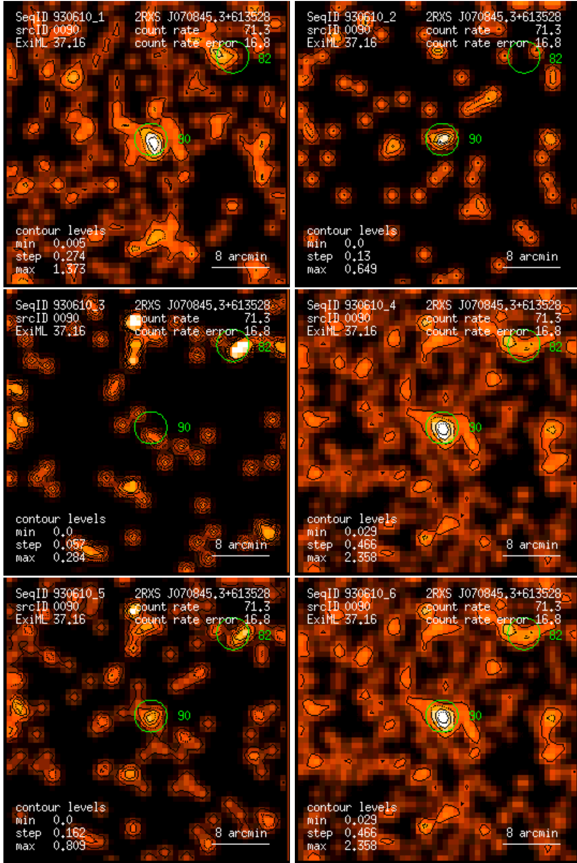
Figure 90: RASS 930610: detection 0090: band rate images, Gaussian filter: (1) PSPC channels 11 – 41, (2) 52 – 90, (3) 91 – 201, (4) 11 – 235, (5) 52 – 201, (6) 11 – 201. Broad band rates in counts/ks. Band rate contour levels in counts/ks/arcmin 2 .
