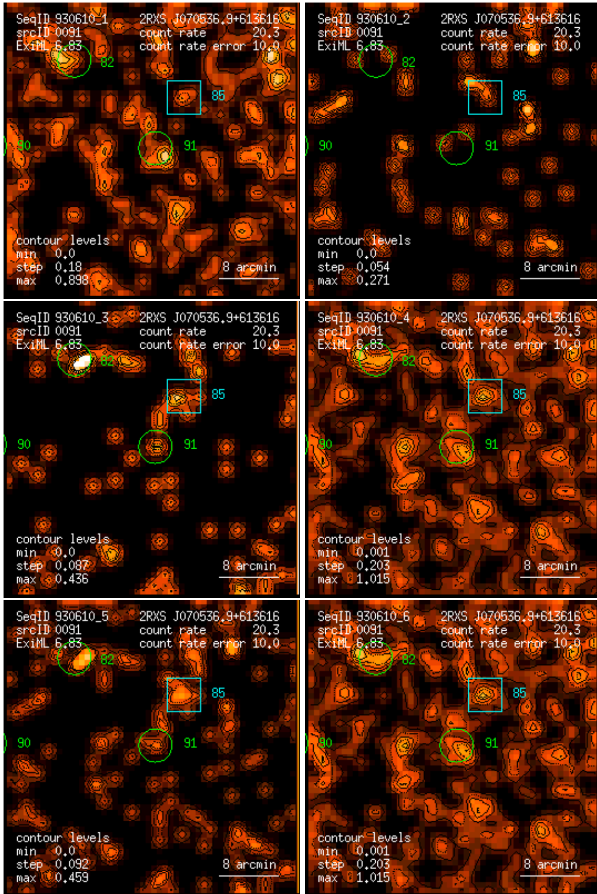
Figure 91: RASS 930610: detection 0091: band rate images, Gaussian filter: (1) PSPC channels 11 – 41, (2) 52 – 90, (3) 91 – 201, (4) 11 – 235, (5) 52 – 201, (6) 11 – 201. Broad band rates in counts/ks. Band rate contour levels in counts/ks/arcmin 2 .
