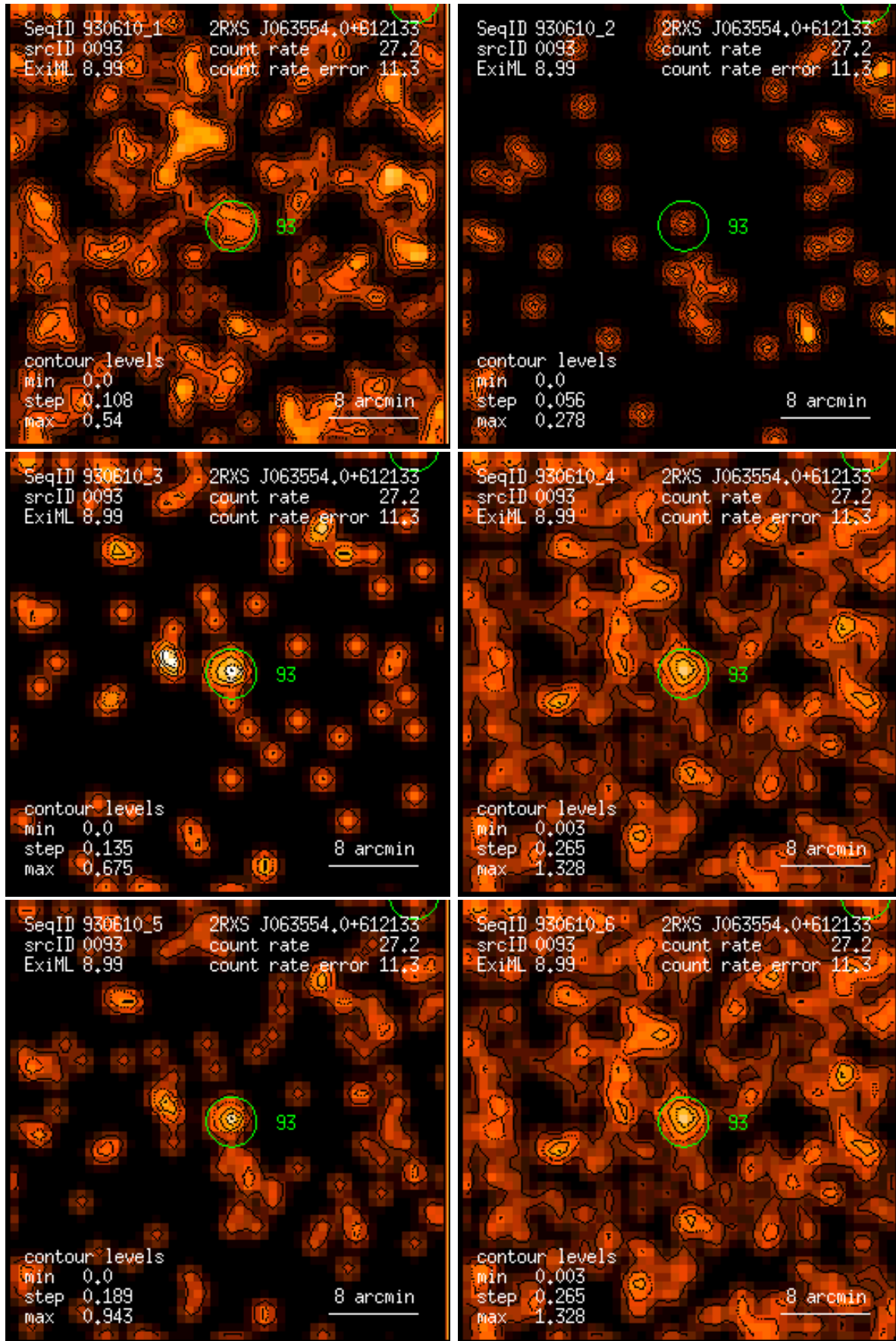
Figure 93: RASS 930610: detection 0093: band rate images, Gaussian filter: (1) PSPC channels 11 – 41, (2) 52 – 90, (3) 91 – 201, (4) 11 – 235, (5) 52 – 201, (6) 11 – 201. Broad band rates in counts/ks. Band rate contour levels in counts/ks/arcmin 2 .
