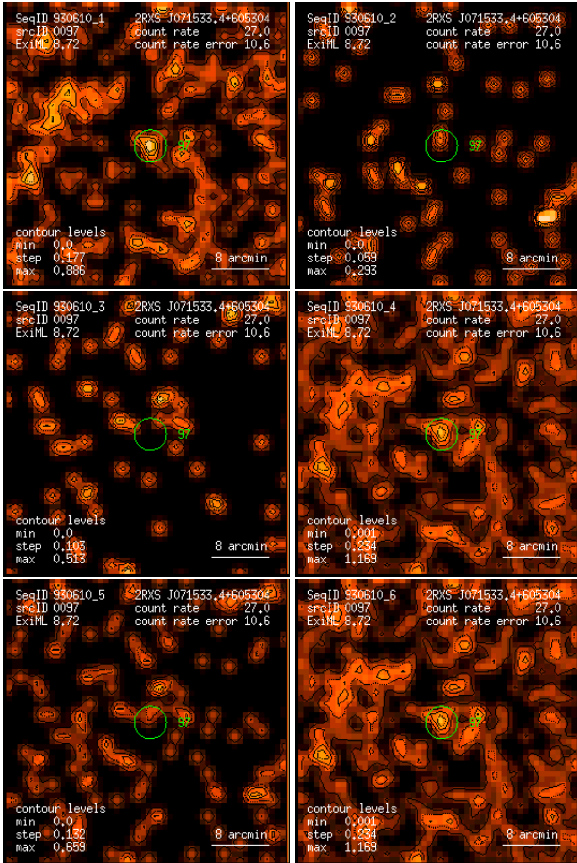
Figure 97: RASS 930610: detection 0097: band rate images, Gaussian filter: (1) PSPC channels 11 – 41, (2) 52 – 90, (3) 91 – 201, (4) 11 – 235, (5) 52 – 201, (6) 11 – 201. Broad band rates in counts/ks. Band rate contour levels in counts/ks/arcmin 2 .
