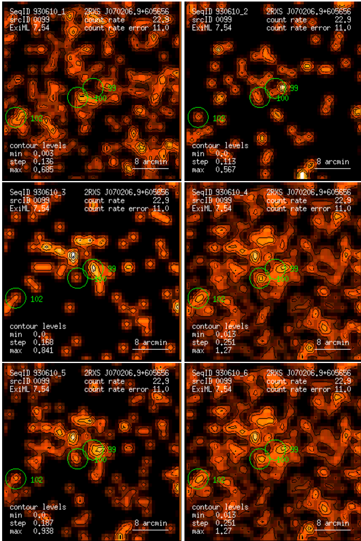
Figure 99: RASS 930610: detection 0099: band rate images, Gaussian filter: (1) PSPC channels 11 – 41, (2) 52 – 90, (3) 91 – 201, (4) 11 – 235, (5) 52 – 201, (6) 11 – 201. Broad band rates in counts/ks. Band rate contour levels in counts/ks/arcmin 2 .
