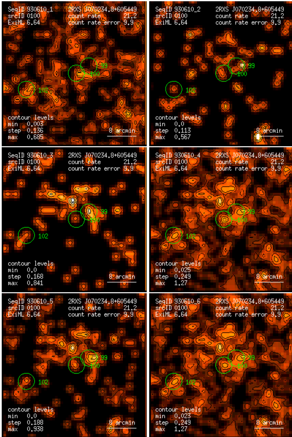
Figure 100: RASS 930610: detection 0100: band rate images, Gaussian filter: (1) PSPC channels 11 – 41, (2) 52 – 90, (3) 91 – 201, (4) 11 – 235, (5) 52 – 201, (6) 11 – 201. Broad band rates in counts/ks. Band rate contour levels in counts/ks/arcmin 2 .
