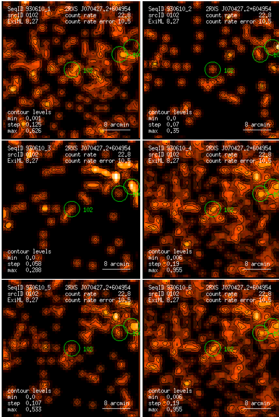
Figure 102: RASS 930610: detection 0102: band rate images, Gaussian filter: (1) PSPC channels 11 – 41, (2) 52 – 90, (3) 91 – 201, (4) 11 – 235, (5) 52 – 201, (6) 11 – 201. Broad band rates in counts/ks. Band rate contour levels in counts/ks/arcmin 2 .
