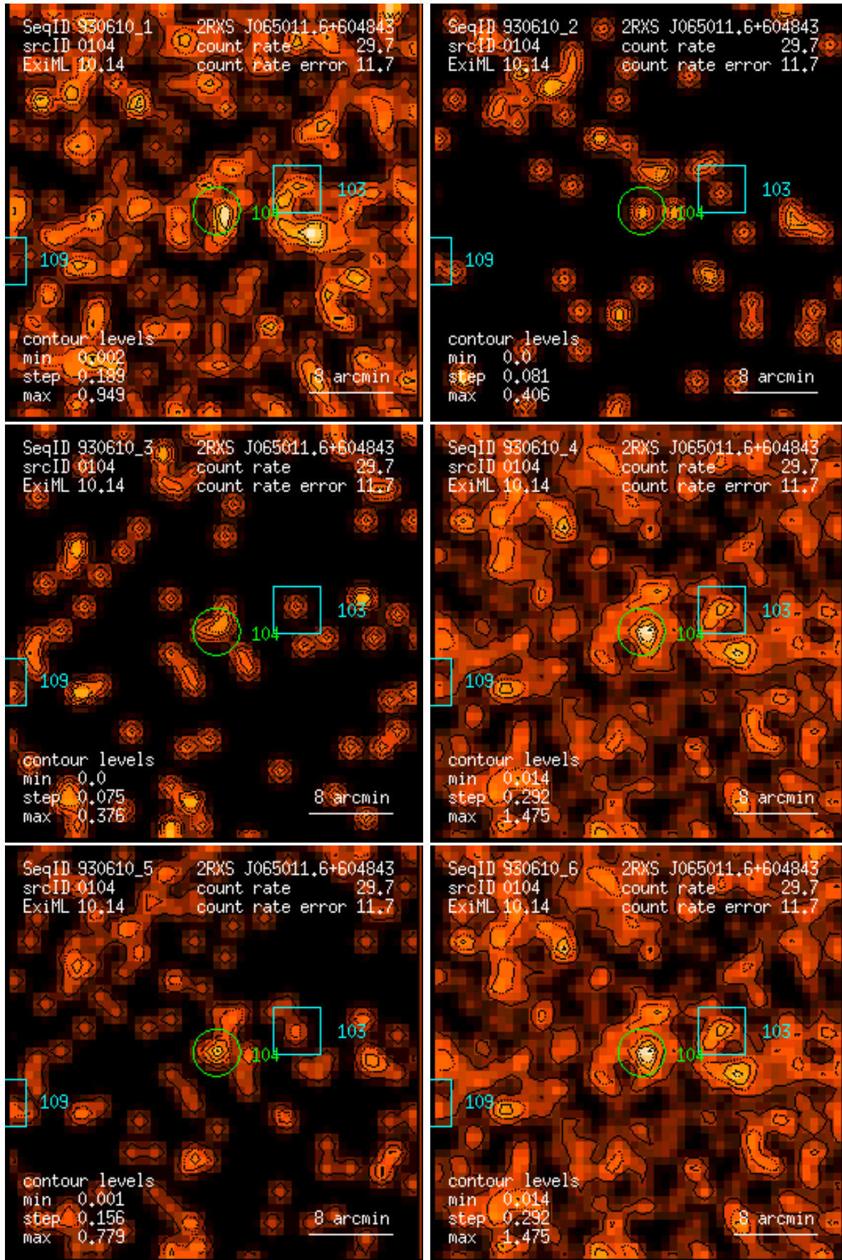
Figure 104: RASS 930610: detection 0104: band rate images, Gaussian filter: (1) PSPC channels 11 – 41, (2) 52 – 90, (3) 91 – 201, (4) 11 – 235, (5) 52 – 201, (6) 11 – 201. Broad band rates in counts/ks. Band rate contour levels in counts/ks/arcmin 2 .
