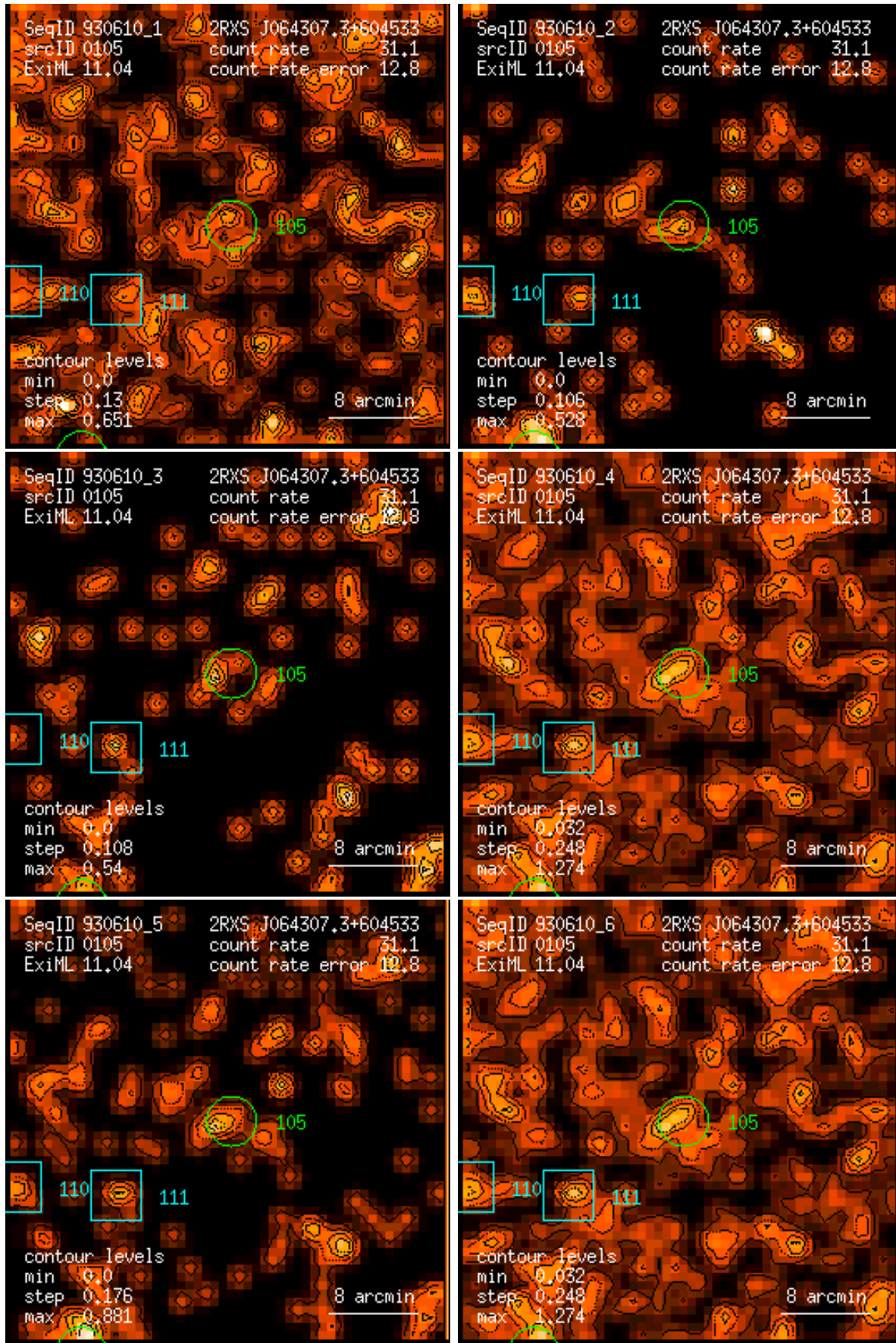
Figure 105: RASS 930610: detection 0105: band rate images, Gaussian filter: (1) PSPC channels 11 – 41, (2) 52 – 90, (3) 91 – 201, (4) 11 – 235, (5) 52 – 201, (6) 11 – 201. Broad band rates in counts/ks. Band rate contour levels in counts/ks/arcmin 2 .
