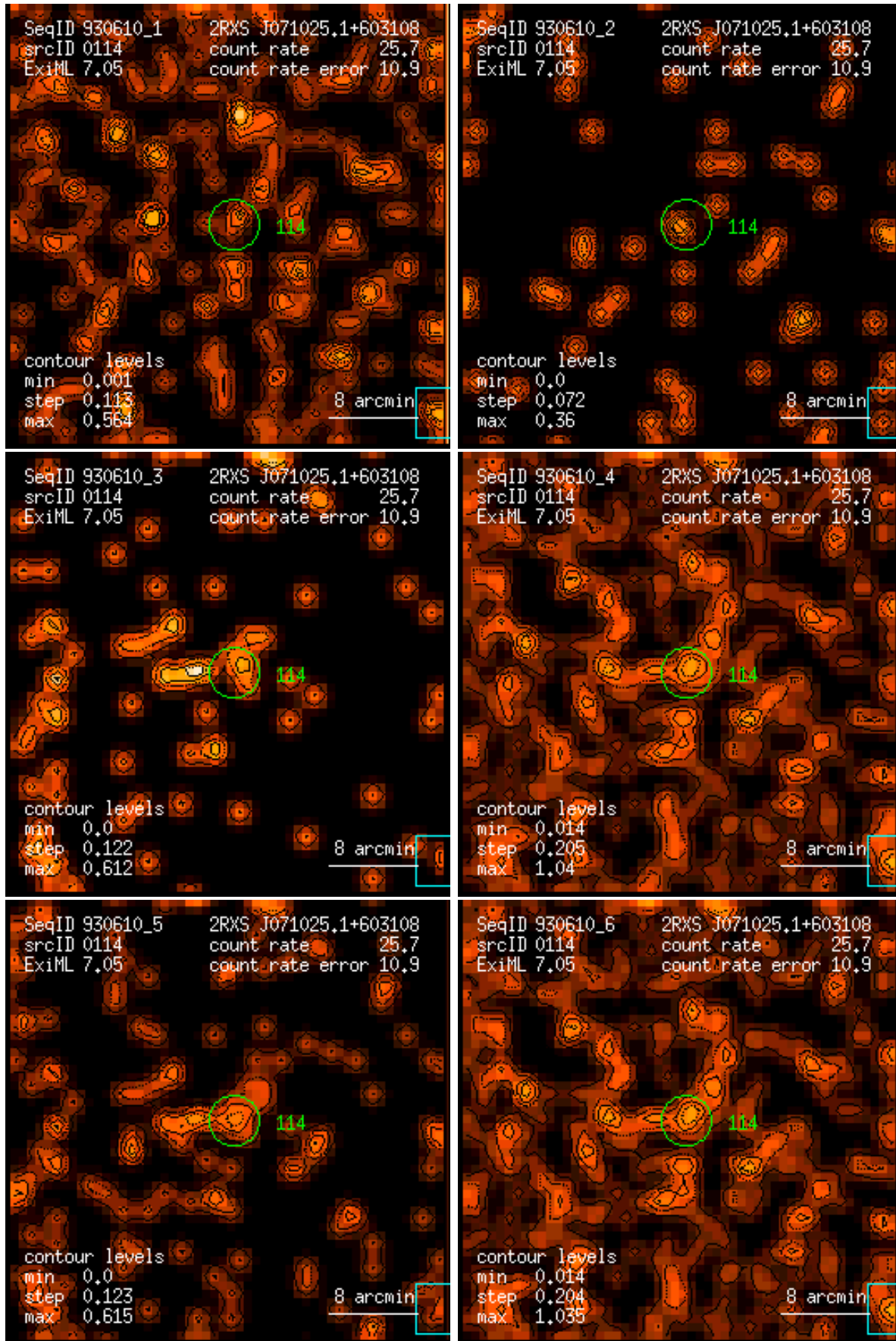
Figure 114: RASS 930610: detection 0114: band rate images, Gaussian filter: (1) PSPC channels 11 – 41, (2) 52 – 90, (3) 91 – 201, (4) 11 – 235, (5) 52 – 201, (6) 11 – 201. Broad band rates in counts/ks. Band rate contour levels in counts/ks/arcmin 2 .
