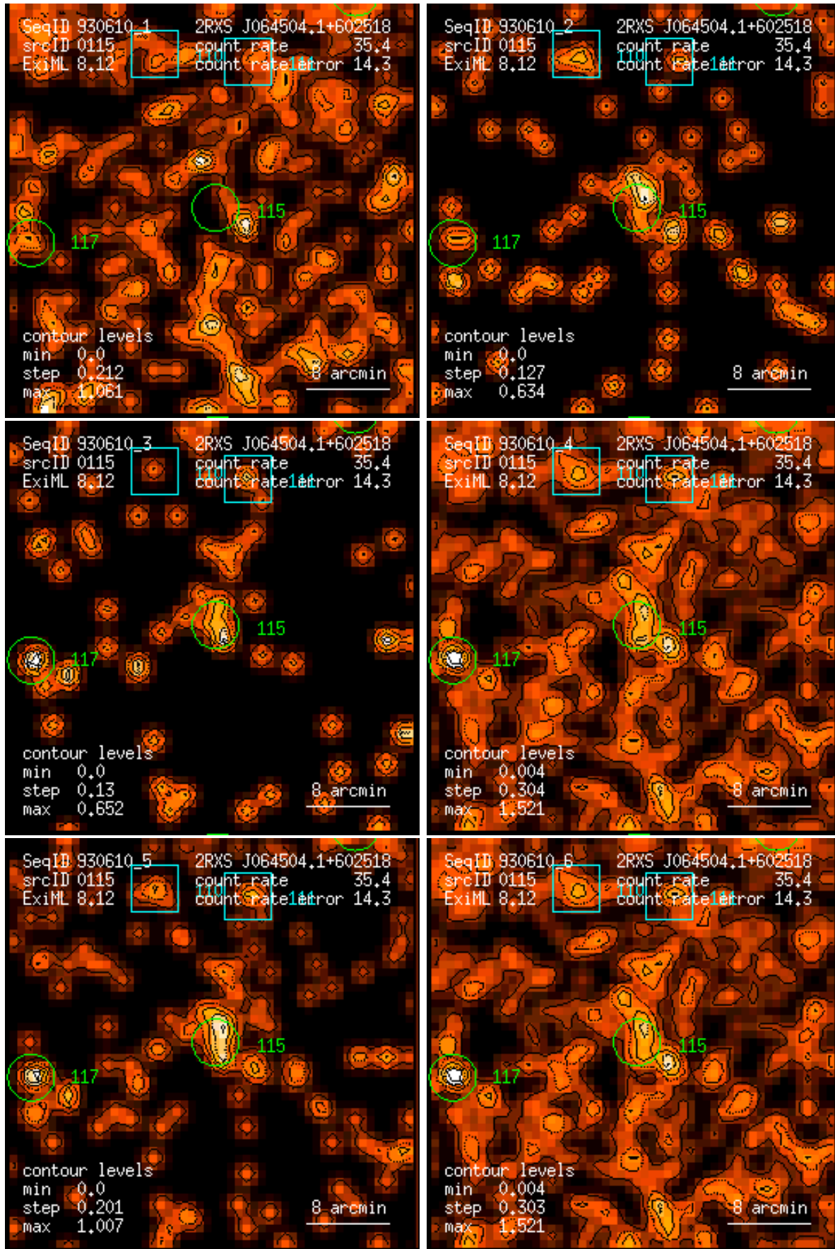
Figure 115: RASS 930610: detection 0115: band rate images, Gaussian filter: (1) PSPC channels 11 – 41, (2) 52 – 90, (3) 91 – 201, (4) 11 – 235, (5) 52 – 201, (6) 11 – 201. Broad band rates in counts/ks. Band rate contour levels in counts/ks/arcmin 2 .
