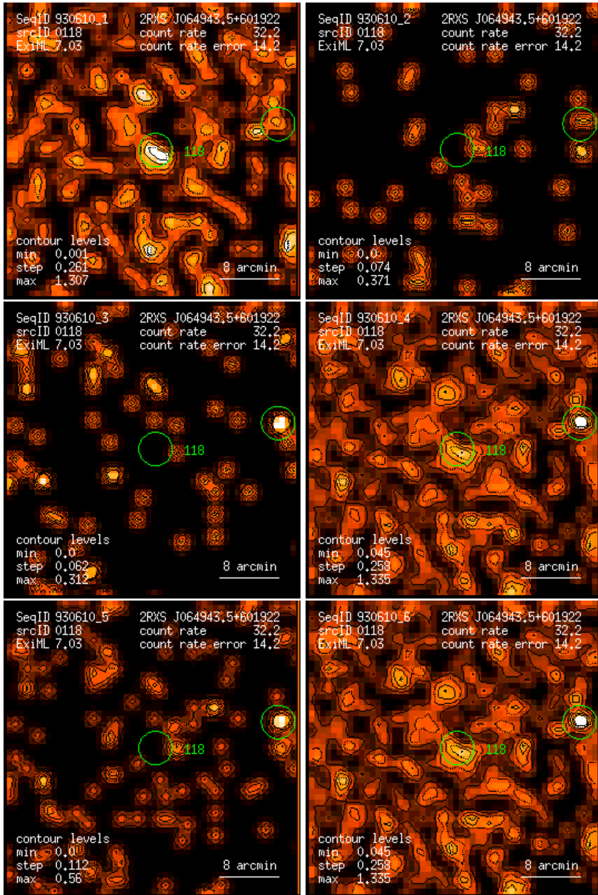
Figure 118: RASS 930610: detection 0118: band rate images, Gaussian filter: (1) PSPC channels 11 – 41, (2) 52 – 90, (3) 91 – 201, (4) 11 – 235, (5) 52 – 201, (6) 11 – 201. Broad band rates in counts/ks. Band rate contour levels in counts/ks/arcmin 2 .
