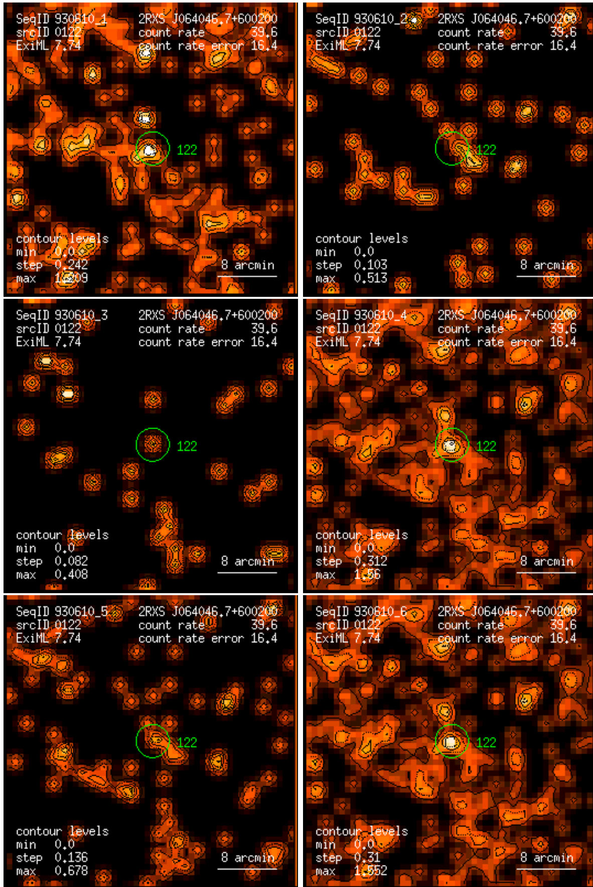
Figure 122: RASS 930610: detection 0122: band rate images, Gaussian filter: (1) PSPC channels 11 – 41, (2) 52 – 90, (3) 91 – 201, (4) 11 – 235, (5) 52 – 201, (6) 11 – 201. Broad band rates in counts/ks. Band rate contour levels in counts/ks/arcmin 2 .
