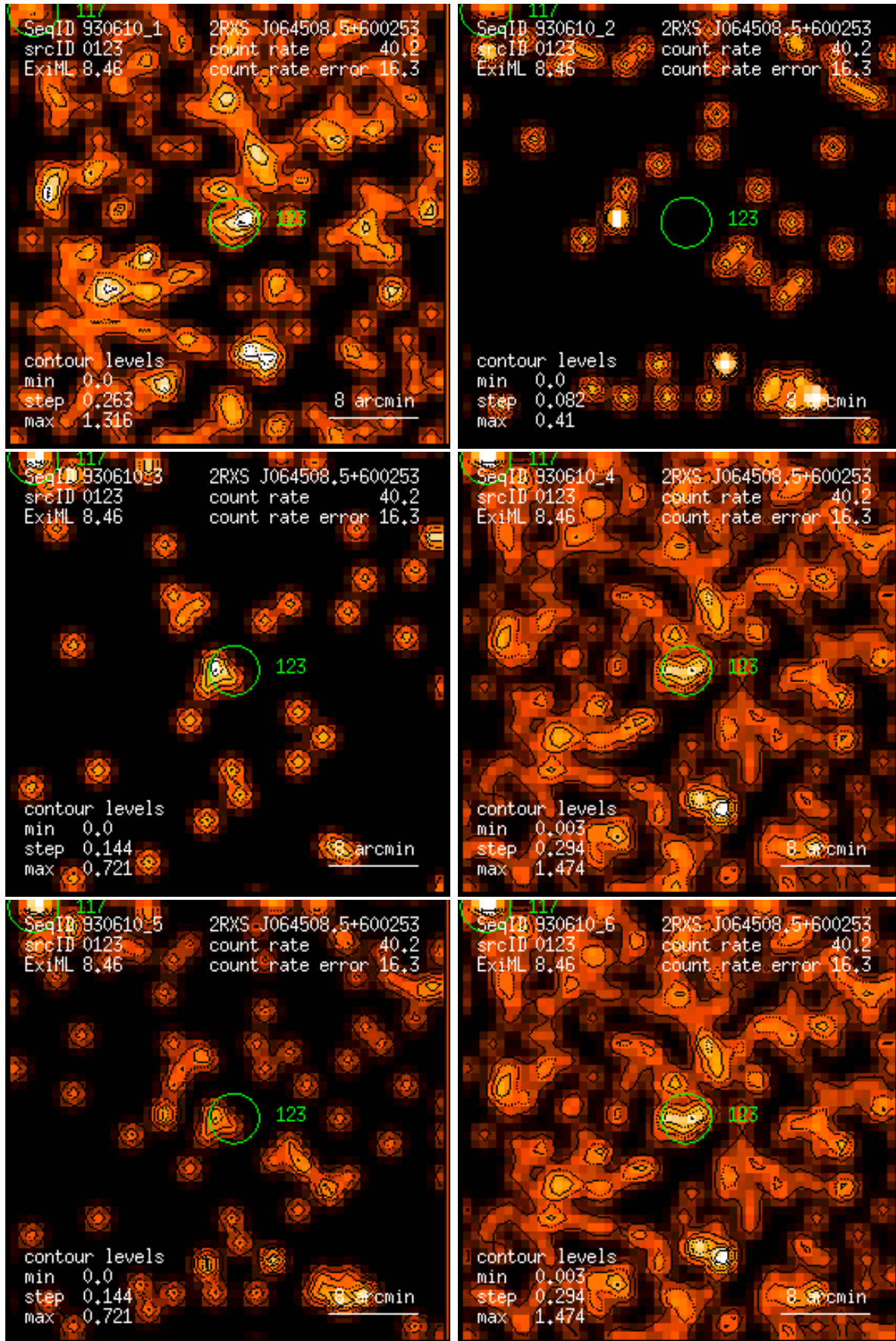
Figure 123: RASS 930610: detection 0123: band rate images, Gaussian filter: (1) PSPC channels 11 – 41, (2) 52 – 90, (3) 91 – 201, (4) 11 – 235, (5) 52 – 201, (6) 11 – 201. Broad band rates in counts/ks. Band rate contour levels in counts/ks/arcmin 2 .
