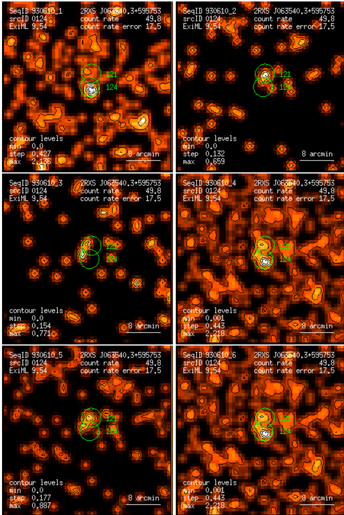
Figure 124: RASS 930610: detection 0124: band rate images, Gaussian filter: (1) PSPC channels 11 – 41, (2) 52 – 90, (3) 91 – 201, (4) 11 – 235, (5) 52 – 201, (6) 11 – 201. Broad band rates in counts/ks. Band rate contour levels in counts/ks/arcmin 2 .
