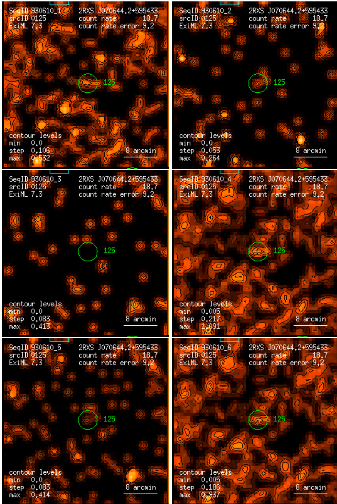
Figure 125: RASS 930610: detection 0125: band rate images, Gaussian filter: (1) PSPC channels 11 – 41, (2) 52 – 90, (3) 91 – 201, (4) 11 – 235, (5) 52 – 201, (6) 11 – 201. Broad band rates in counts/ks. Band rate contour levels in counts/ks/arcmin 2 .
