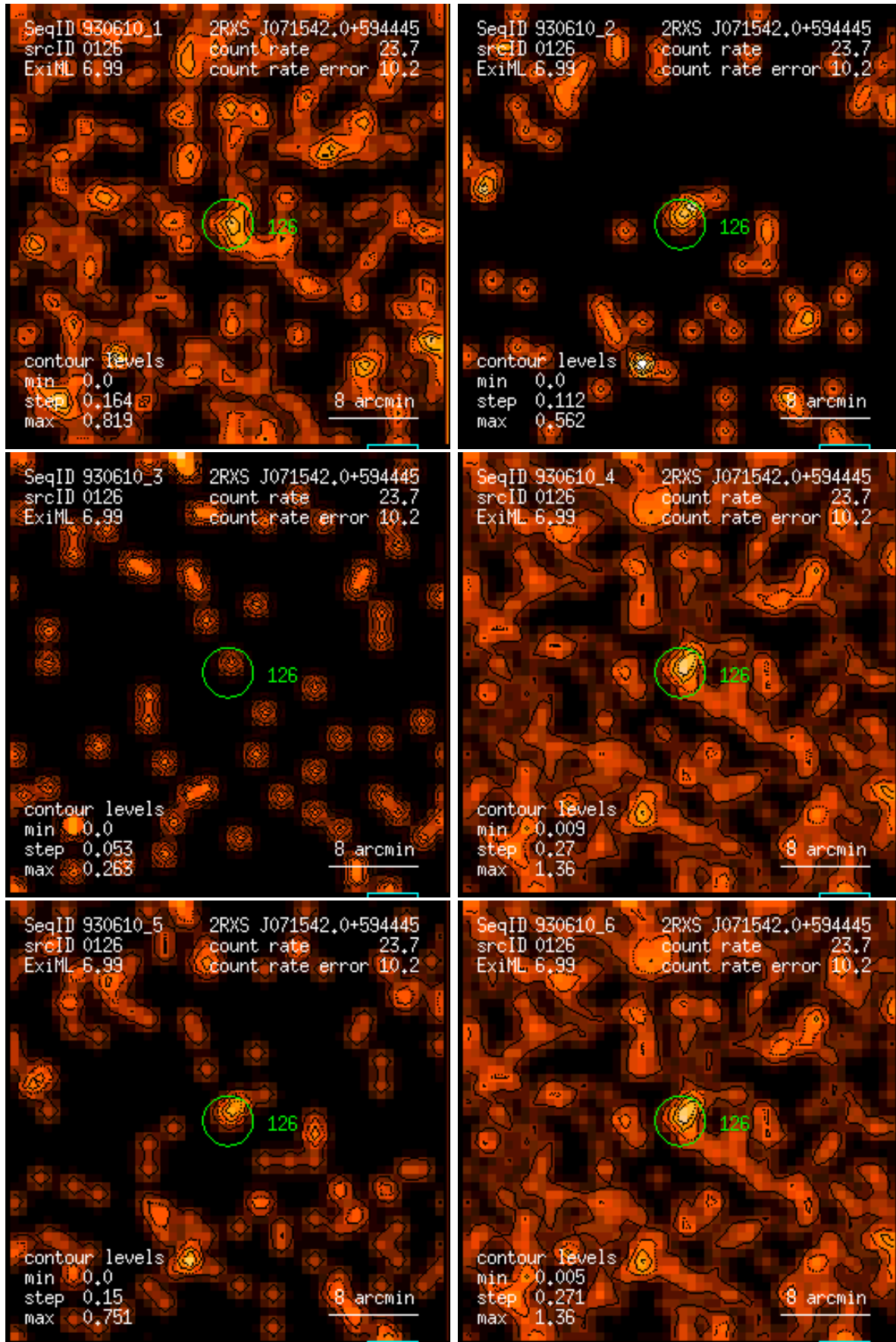
Figure 126: RASS 930610: detection 0126: band rate images, Gaussian filter: (1) PSPC channels 11 – 41, (2) 52 – 90, (3) 91 – 201, (4) 11 – 235, (5) 52 – 201, (6) 11 – 201. Broad band rates in counts/ks. Band rate contour levels in counts/ks/arcmin 2 .
