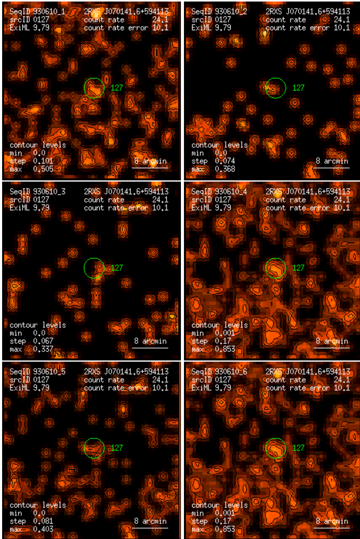
Figure 127: RASS 930610: detection 0127: band rate images, Gaussian filter: (1) PSPC channels 11 – 41, (2) 52 – 90, (3) 91 – 201, (4) 11 – 235, (5) 52 – 201, (6) 11 – 201. Broad band rates in counts/ks. Band rate contour levels in counts/ks/arcmin 2 .
