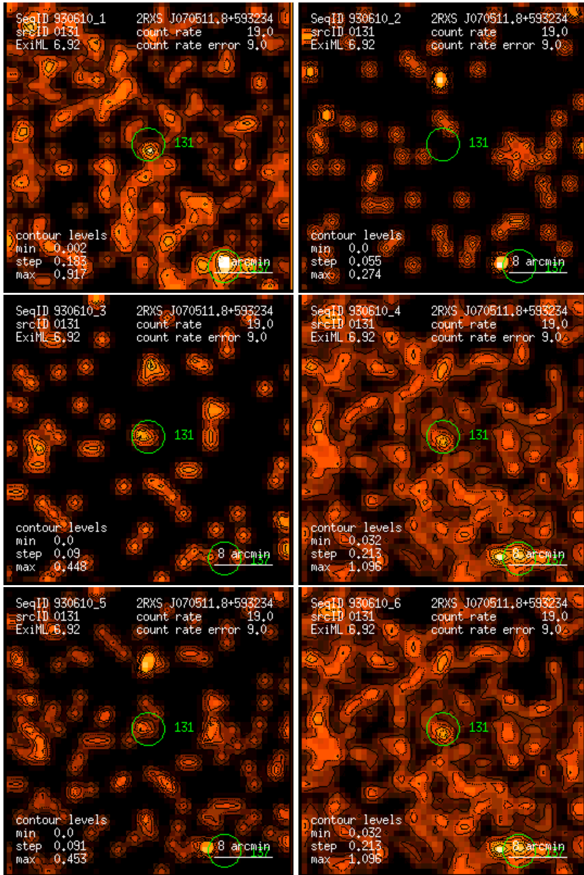
Figure 131: RASS 930610: detection 0131: band rate images, Gaussian filter: (1) PSPC channels 11 – 41, (2) 52 – 90, (3) 91 – 201, (4) 11 – 235, (5) 52 – 201, (6) 11 – 201. Broad band rates in counts/ks. Band rate contour levels in counts/ks/arcmin 2 .
