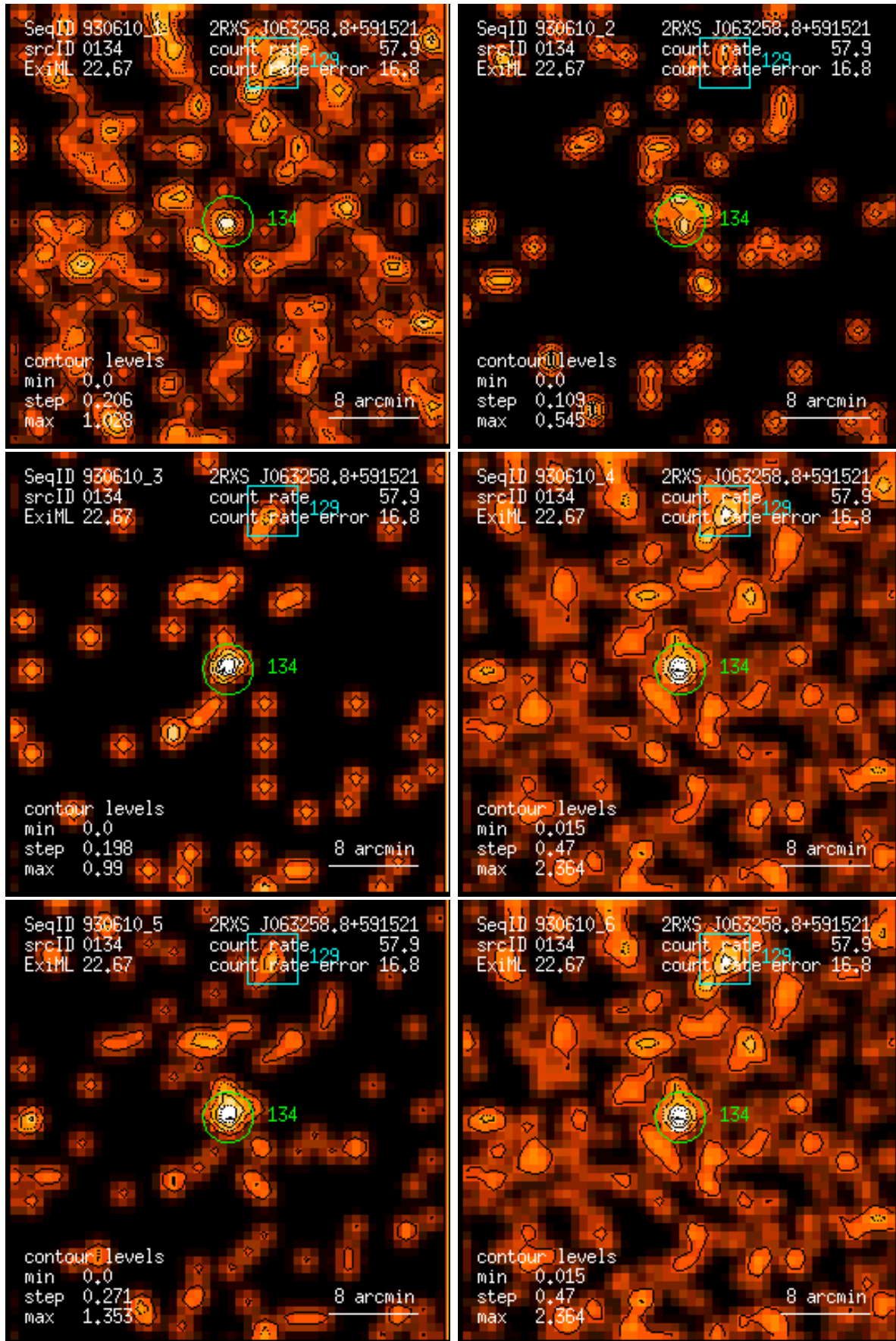
Figure 134: RASS 930610: detection 0134: band rate images, Gaussian filter: (1) PSPC channels 11 – 41, (2) 52 – 90, (3) 91 – 201, (4) 11 – 235, (5) 52 – 201, (6) 11 – 201. Broad band rates in counts/ks. Band rate contour levels in counts/ks/arcmin 2 .
